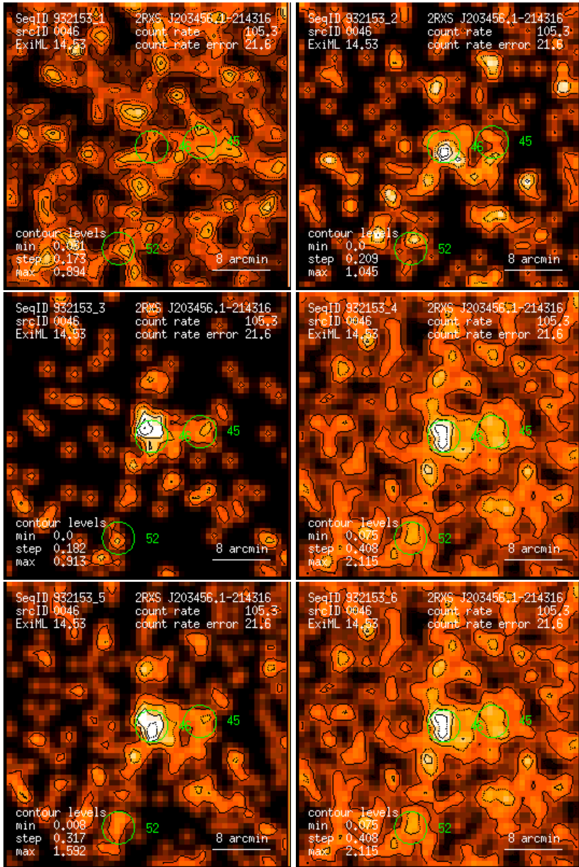
Figure 46: RASS 932153: detection 0046: band rate images, Gaussian filter: (1) PSPC channels 11 – 41, (2) 52 – 90, (3) 91 – 201, (4) 11 – 235, (5) 52 – 201, (6) 11 – 201. Broad band rates in counts/ks. Band rate contour levels in counts/ks/arcmin 2 .
