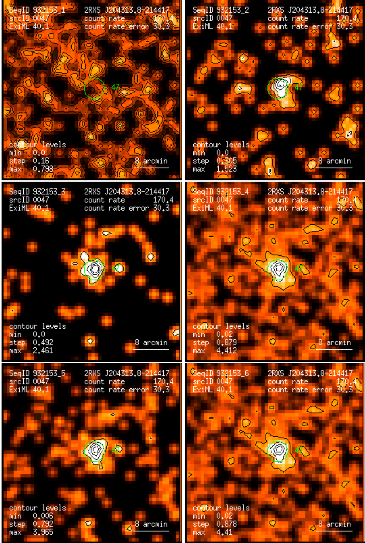
Figure 47: RASS 932153: detection 0047: band rate images, Gaussian filter: (1) PSPC channels 11 – 41, (2) 52 – 90, (3) 91 – 201, (4) 11 – 235, (5) 52 – 201, (6) 11 – 201. Broad band rates in counts/ks. Band rate contour levels in counts/ks/arcmin 2 .
