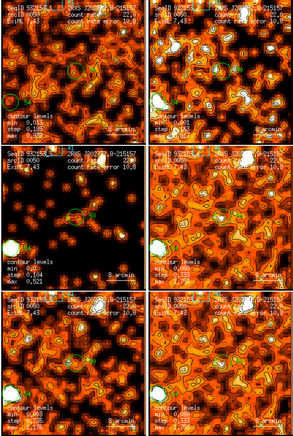
Figure 50: RASS 932153: detection 0050: band rate images, Gaussian filter: (1) PSPC channels 11 – 41, (2) 52 – 90, (3) 91 – 201, (4) 11 – 235, (5) 52 – 201, (6) 11 – 201. Broad band rates in counts/ks. Band rate contour levels in counts/ks/arcmin 2 .
