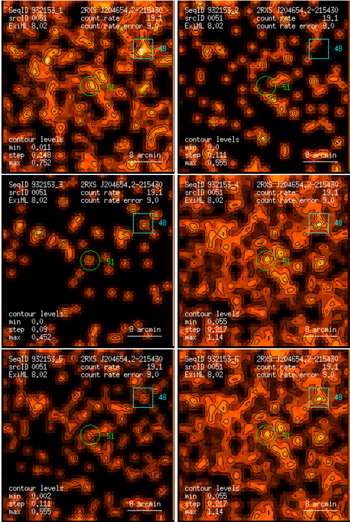
Figure 51: RASS 932153: detection 0051: band rate images, Gaussian filter: (1) PSPC channels 11 – 41, (2) 52 – 90, (3) 91 – 201, (4) 11 – 235, (5) 52 – 201, (6) 11 – 201. Broad band rates in counts/ks. Band rate contour levels in counts/ks/arcmin 2 .
