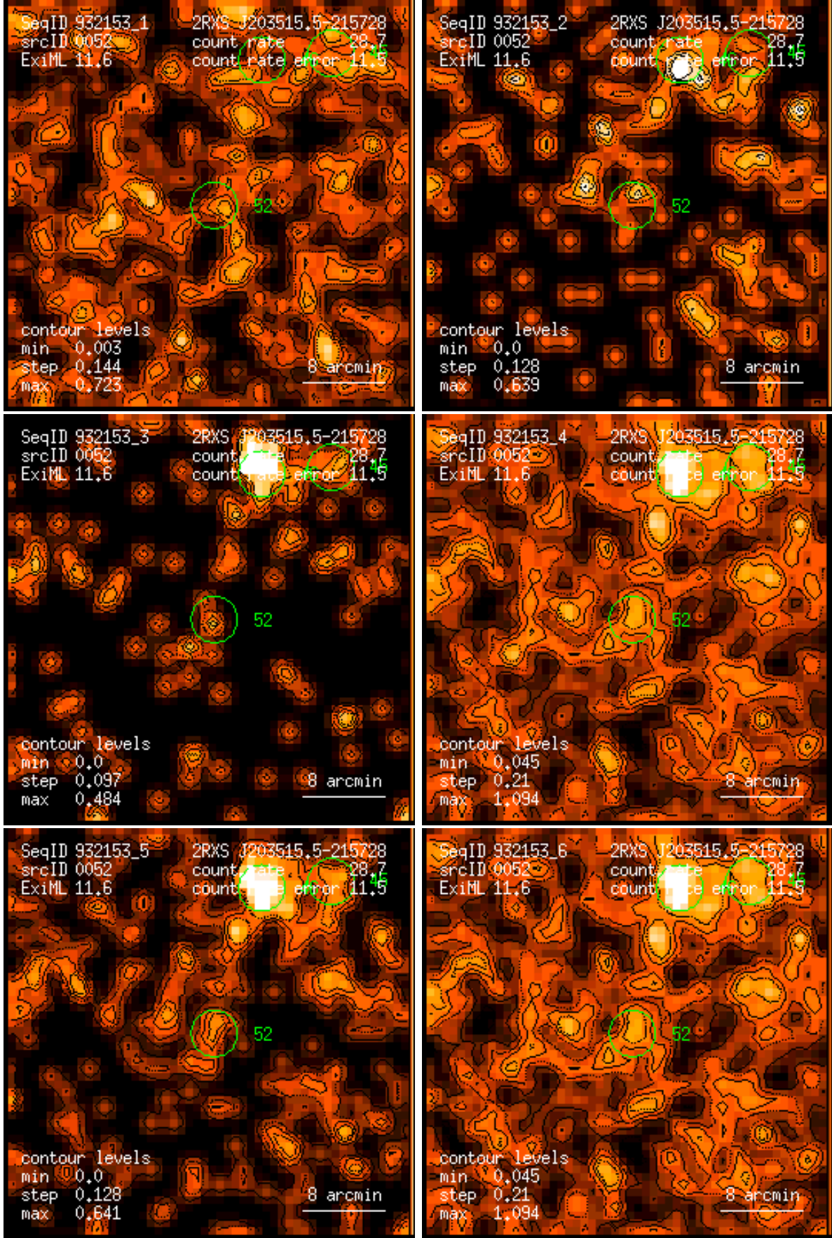
Figure 52: RASS 932153: detection 0052: band rate images, Gaussian filter: (1) PSPC channels 11 – 41, (2) 52 – 90, (3) 91 – 201, (4) 11 – 235, (5) 52 – 201, (6) 11 – 201. Broad band rates in counts/ks. Band rate contour levels in counts/ks/arcmin 2 .
