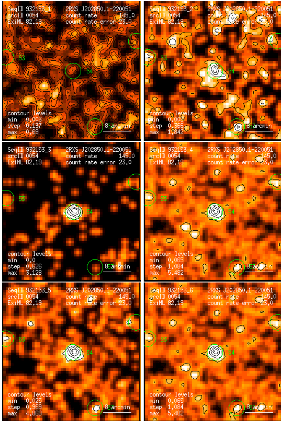
Figure 54: RASS 932153: detection 0054: band rate images, Gaussian filter: (1) PSPC channels 11 – 41, (2) 52 – 90, (3) 91 – 201, (4) 11 – 235, (5) 52 – 201, (6) 11 – 201. Broad band rates in counts/ks. Band rate contour levels in counts/ks/arcmin 2 .
