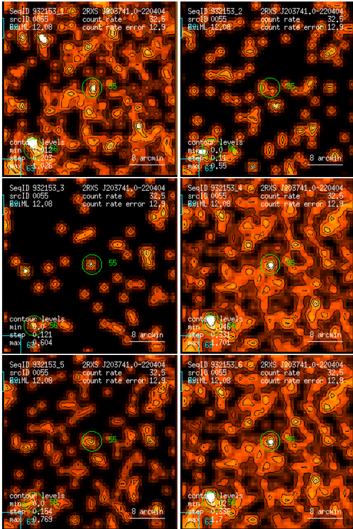
Figure 55: RASS 932153: detection 0055: band rate images, Gaussian filter: (1) PSPC channels 11 – 41, (2) 52 – 90, (3) 91 – 201, (4) 11 – 235, (5) 52 – 201, (6) 11 – 201. Broad band rates in counts/ks. Band rate contour levels in counts/ks/arcmin 2 .
