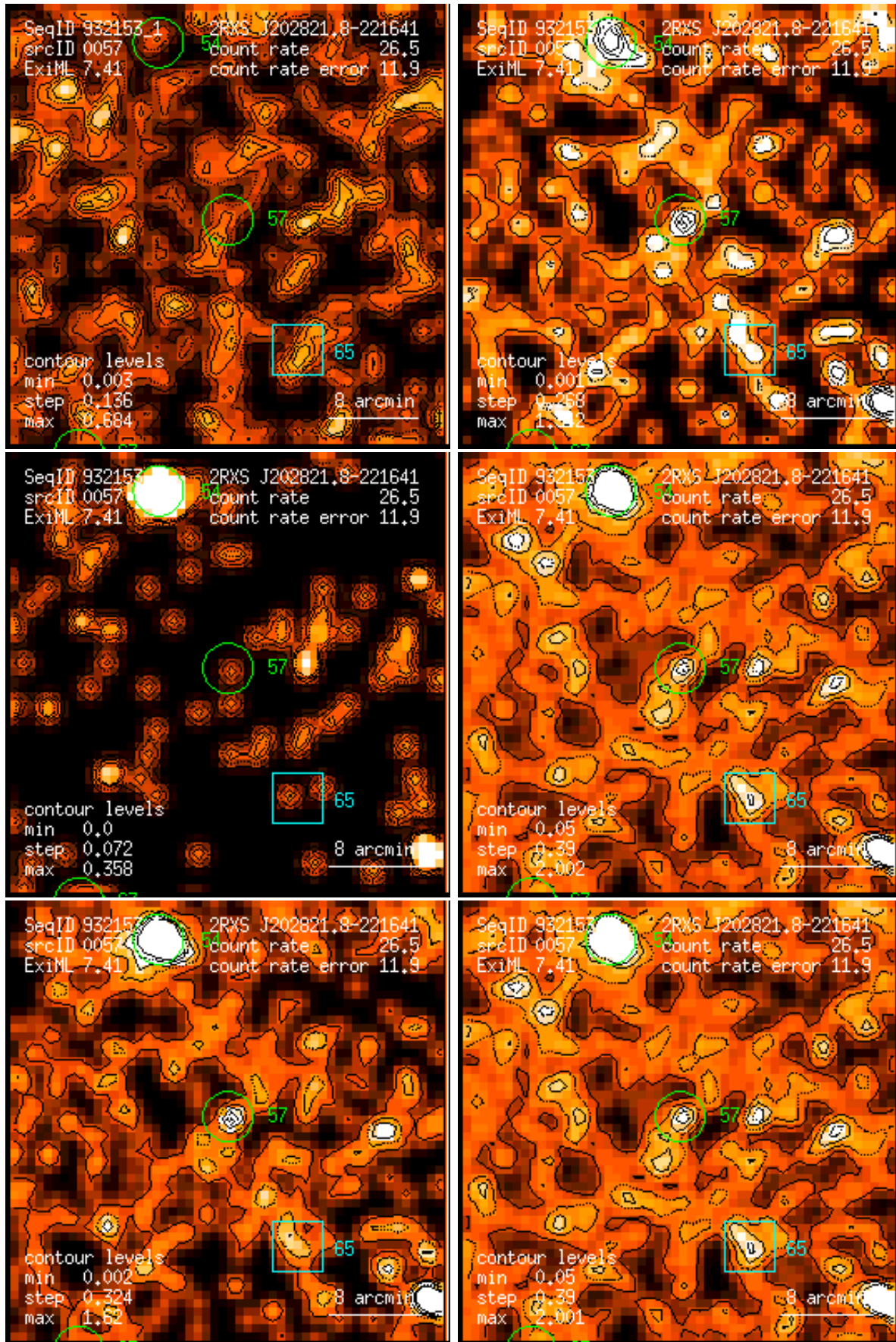
Figure 57: RASS 932153: detection 0057: band rate images, Gaussian filter: (1) PSPC channels 11 – 41, (2) 52 – 90, (3) 91 – 201, (4) 11 – 235, (5) 52 – 201, (6) 11 – 201. Broad band rates in counts/ks. Band rate contour levels in counts/ks/arcmin 2 .
