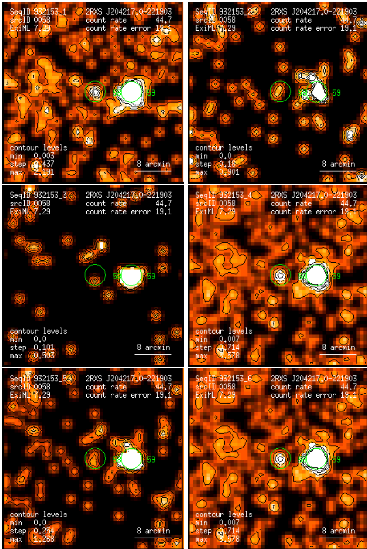
Figure 58: RASS 932153: detection 0058: band rate images, Gaussian filter: (1) PSPC channels 11 – 41, (2) 52 – 90, (3) 91 – 201, (4) 11 – 235, (5) 52 – 201, (6) 11 – 201. Broad band rates in counts/ks. Band rate contour levels in counts/ks/arcmin 2 .
