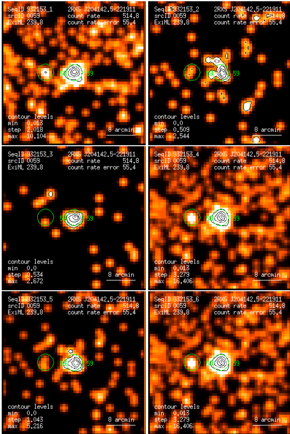
Figure 59: RASS 932153: detection 0059: band rate images, Gaussian filter: (1) PSPC channels 11 – 41, (2) 52 – 90, (3) 91 – 201, (4) 11 – 235, (5) 52 – 201, (6) 11 – 201. Broad band rates in counts/ks. Band rate contour levels in counts/ks/arcmin 2 .
