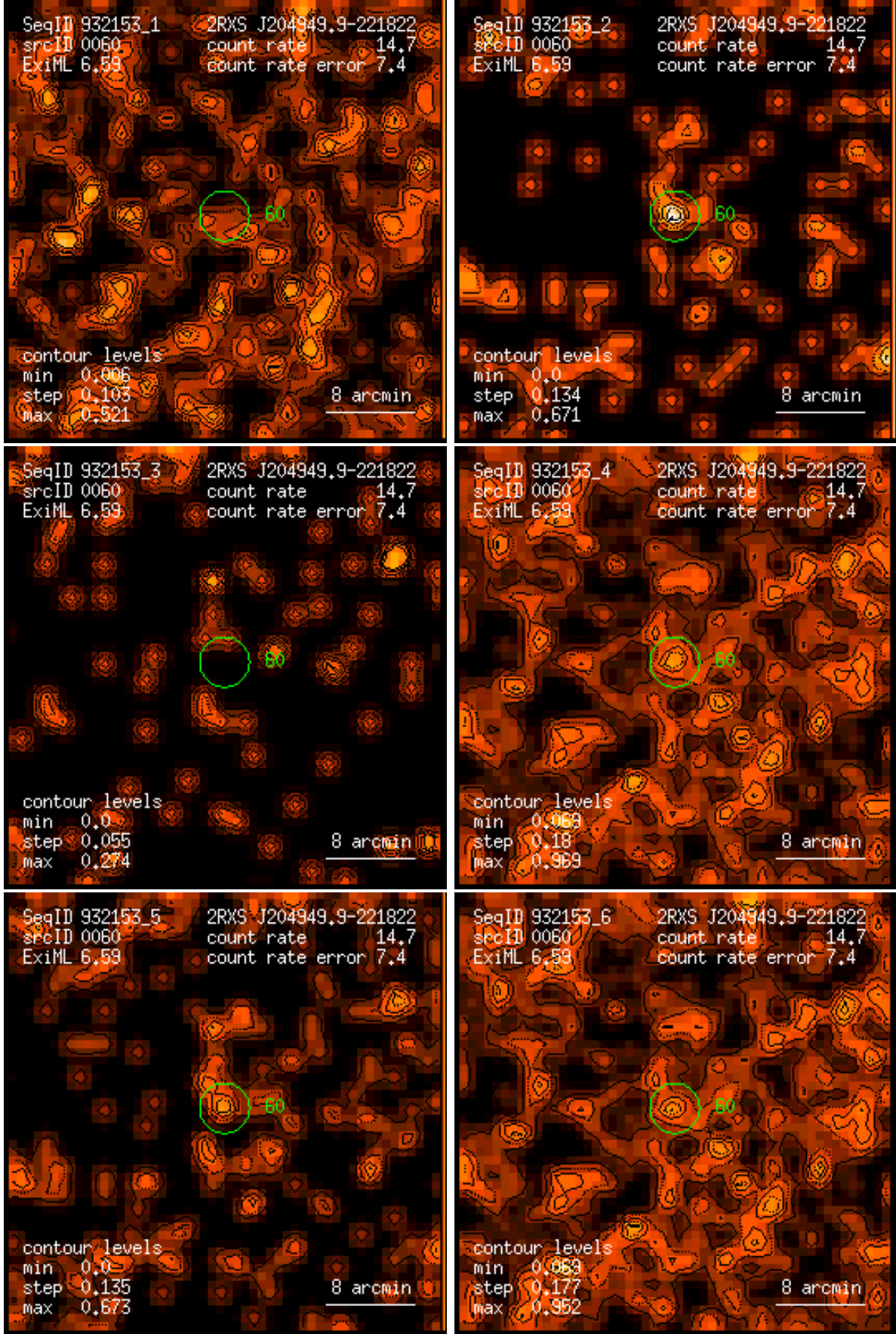
Figure 60: RASS 932153: detection 0060: band rate images, Gaussian filter: (1) PSPC channels 11 – 41, (2) 52 – 90, (3) 91 – 201, (4) 11 – 235, (5) 52 – 201, (6) 11 – 201. Broad band rates in counts/ks. Band rate contour levels in counts/ks/arcmin 2 .
