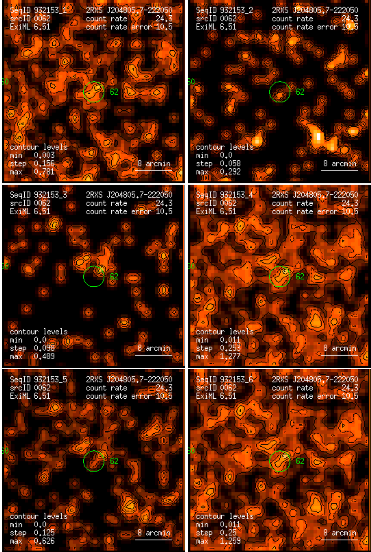
Figure 62: RASS 932153: detection 0062: band rate images, Gaussian filter: (1) PSPC channels 11 – 41, (2) 52 – 90, (3) 91 – 201, (4) 11 – 235, (5) 52 – 201, (6) 11 – 201. Broad band rates in counts/ks. Band rate contour levels in counts/ks/arcmin 2 .
