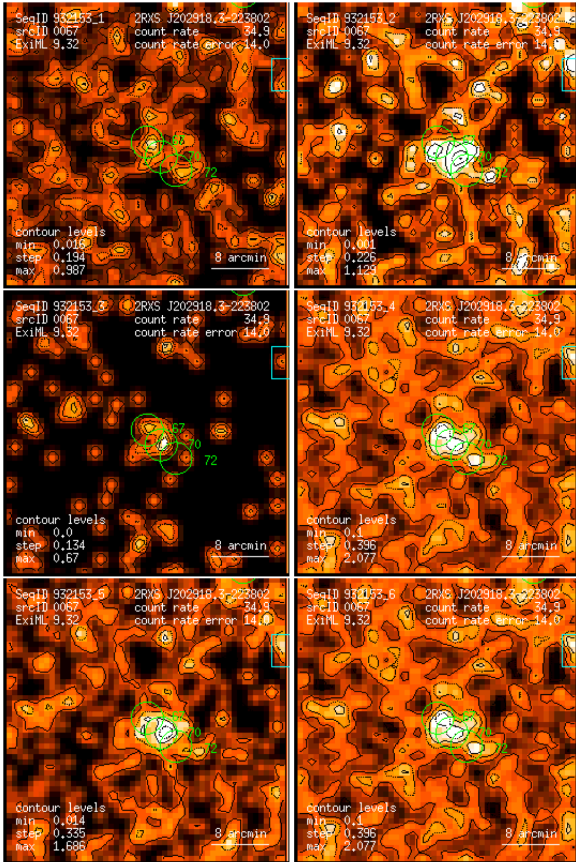
Figure 67: RASS 932153: detection 0067: band rate images, Gaussian filter: (1) PSPC channels 11 – 41, (2) 52 – 90, (3) 91 – 201, (4) 11 – 235, (5) 52 – 201, (6) 11 – 201. Broad band rates in counts/ks. Band rate contour levels in counts/ks/arcmin 2 .
