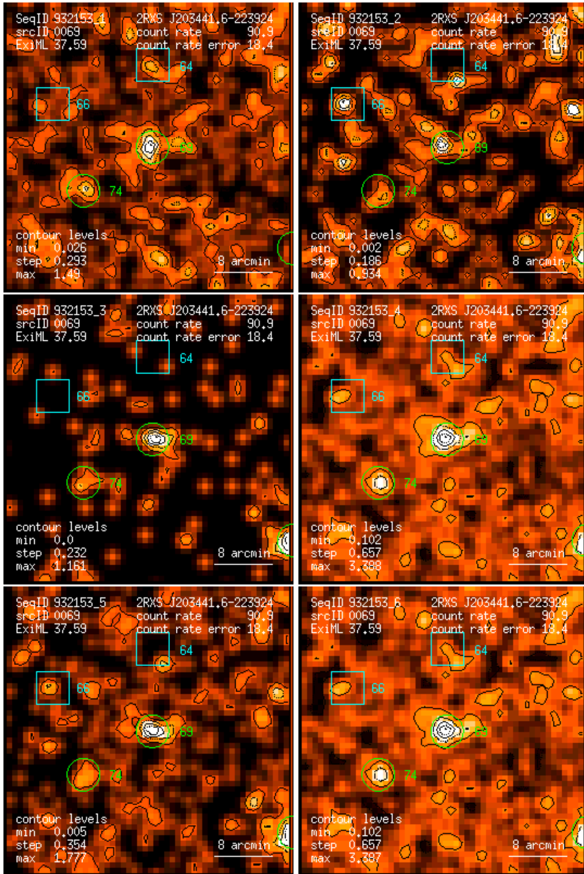
Figure 69: RASS 932153: detection 0069: band rate images, Gaussian filter: (1) PSPC channels 11 – 41, (2) 52 – 90, (3) 91 – 201, (4) 11 – 235, (5) 52 – 201, (6) 11 – 201. Broad band rates in counts/ks. Band rate contour levels in counts/ks/arcmin 2 .
