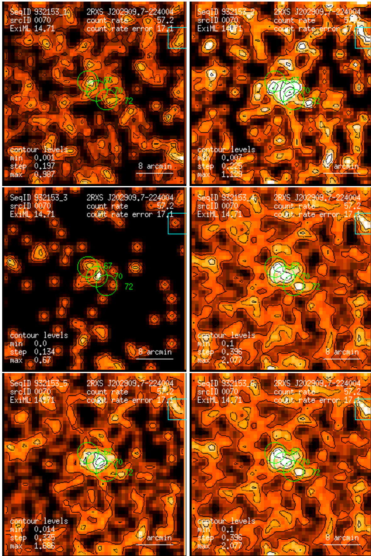
Figure 70: RASS 932153: detection 0070: band rate images, Gaussian filter: (1) PSPC channels 11 – 41, (2) 52 – 90, (3) 91 – 201, (4) 11 – 235, (5) 52 – 201, (6) 11 – 201. Broad band rates in counts/ks. Band rate contour levels in counts/ks/arcmin 2 .
