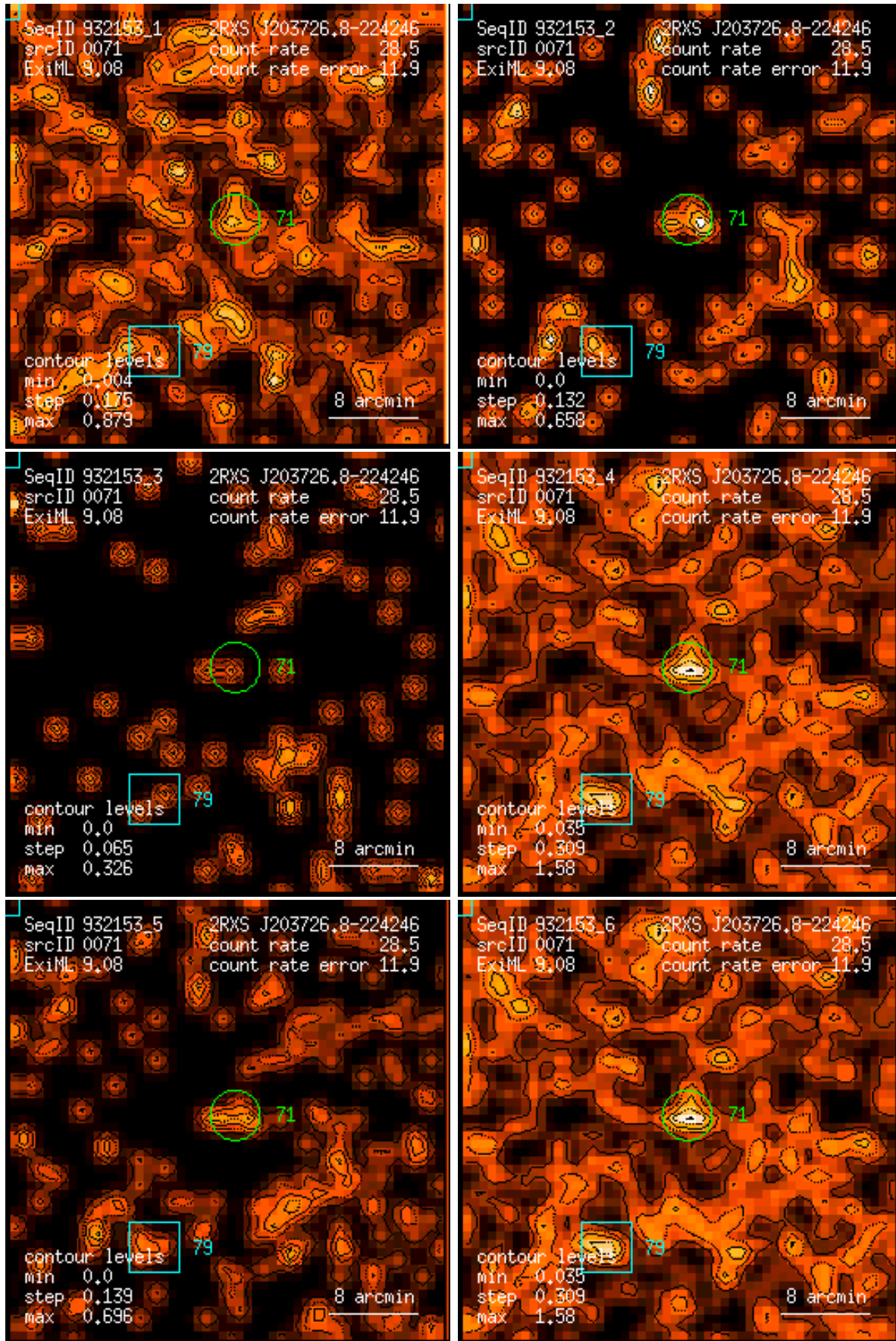
Figure 71: RASS 932153: detection 0071: band rate images, Gaussian filter: (1) PSPC channels 11 – 41, (2) 52 – 90, (3) 91 – 201, (4) 11 – 235, (5) 52 – 201, (6) 11 – 201. Broad band rates in counts/ks. Band rate contour levels in counts/ks/arcmin 2 .
