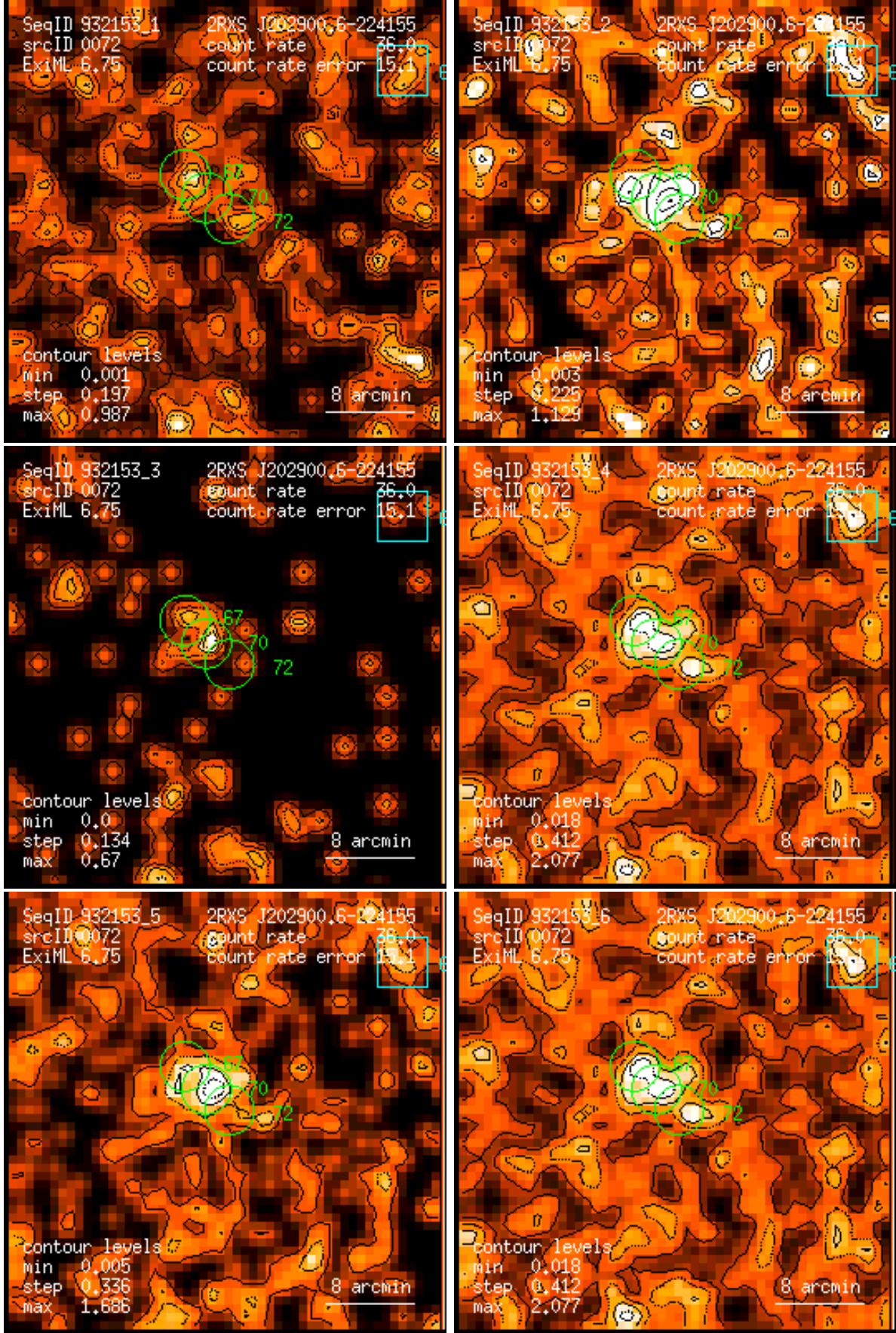
Figure 72: RASS 932153: detection 0072: band rate images, Gaussian filter: (1) PSPC channels 11 – 41, (2) 52 – 90, (3) 91 – 201, (4) 11 – 235, (5) 52 – 201, (6) 11 – 201. Broad band rates in counts/ks. Band rate contour levels in counts/ks/arcmin 2 .
