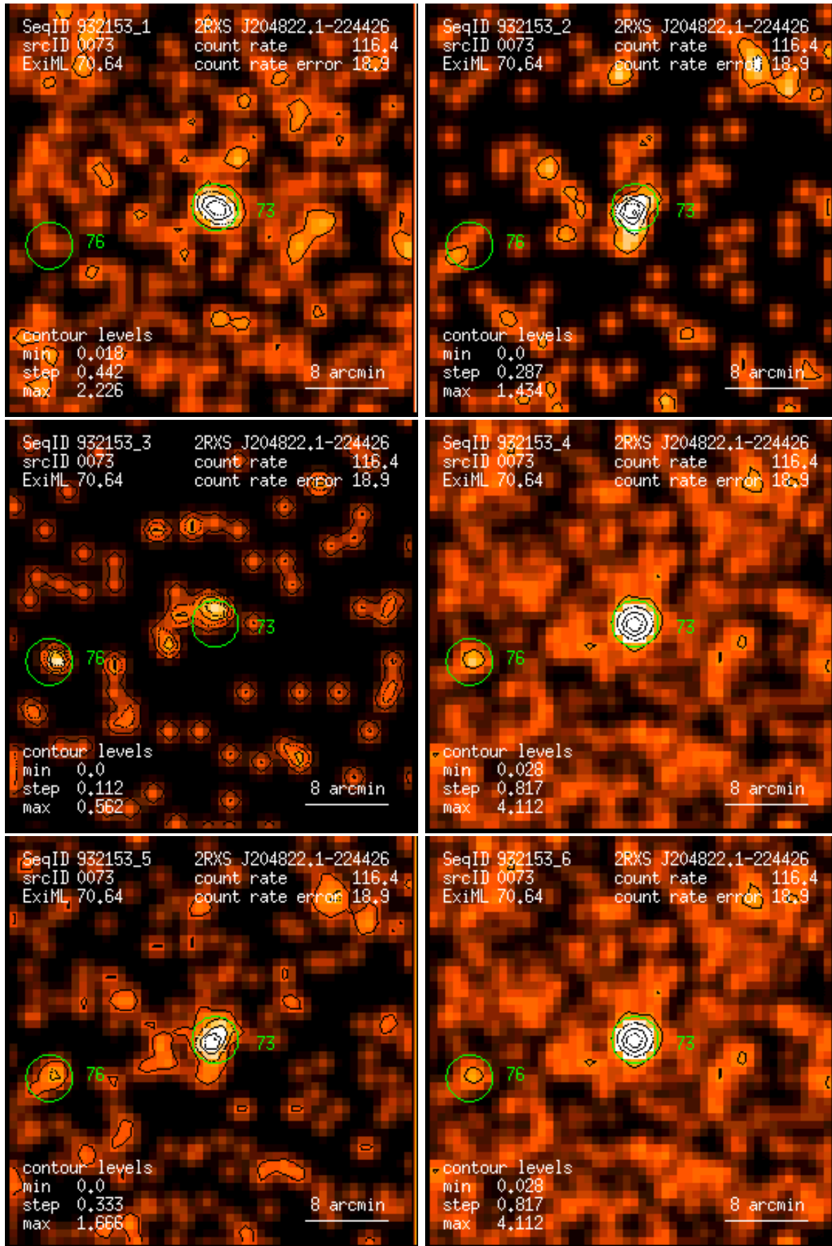
Figure 73: RASS 932153: detection 0073: band rate images, Gaussian filter: (1) PSPC channels 11 – 41, (2) 52 – 90, (3) 91 – 201, (4) 11 – 235, (5) 52 – 201, (6) 11 – 201. Broad band rates in counts/ks. Band rate contour levels in counts/ks/arcmin 2 .
