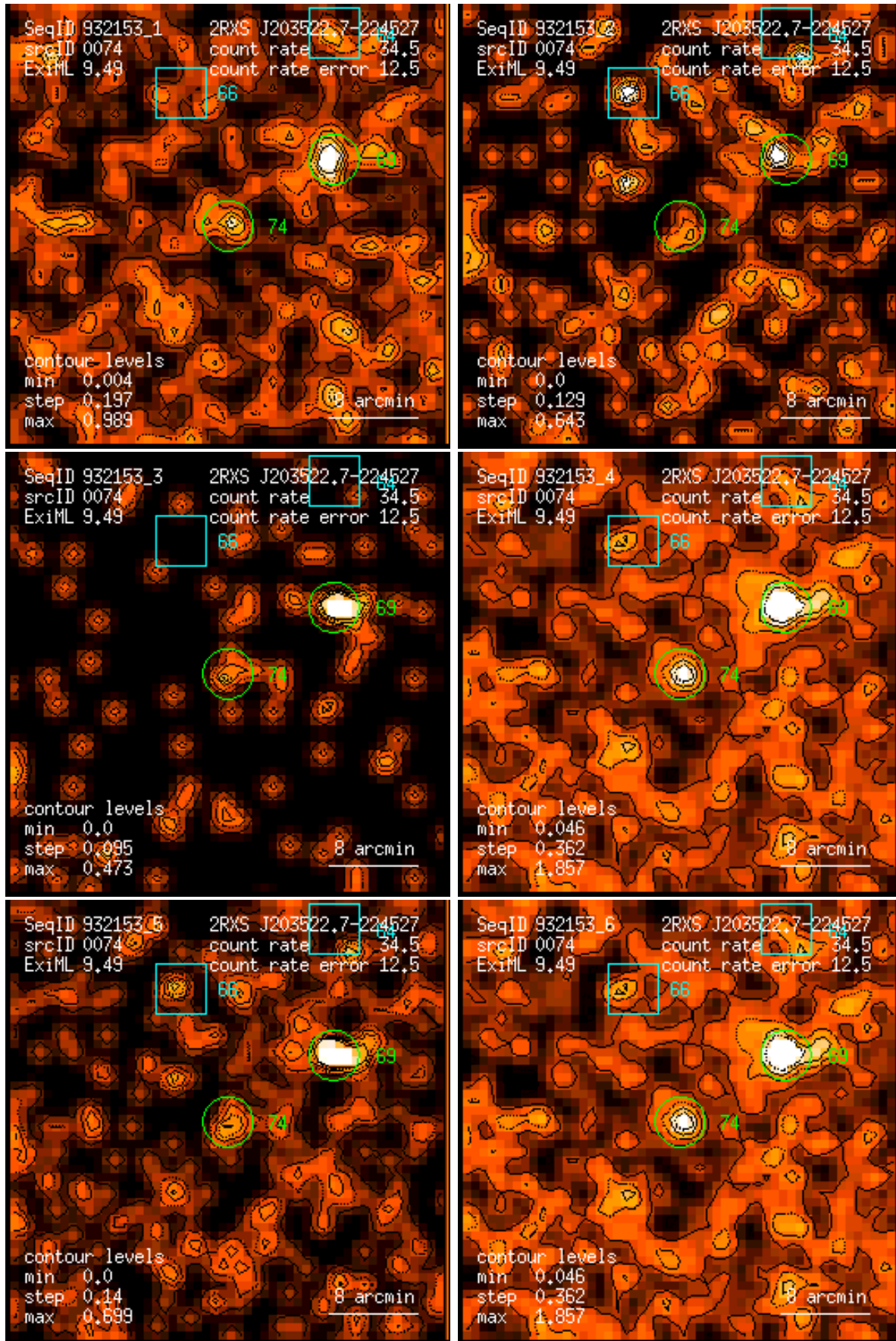
Figure 74: RASS 932153: detection 0074: band rate images, Gaussian filter: (1) PSPC channels 11 – 41, (2) 52 – 90, (3) 91 – 201, (4) 11 – 235, (5) 52 – 201, (6) 11 – 201. Broad band rates in counts/ks. Band rate contour levels in counts/ks/arcmin 2 .
