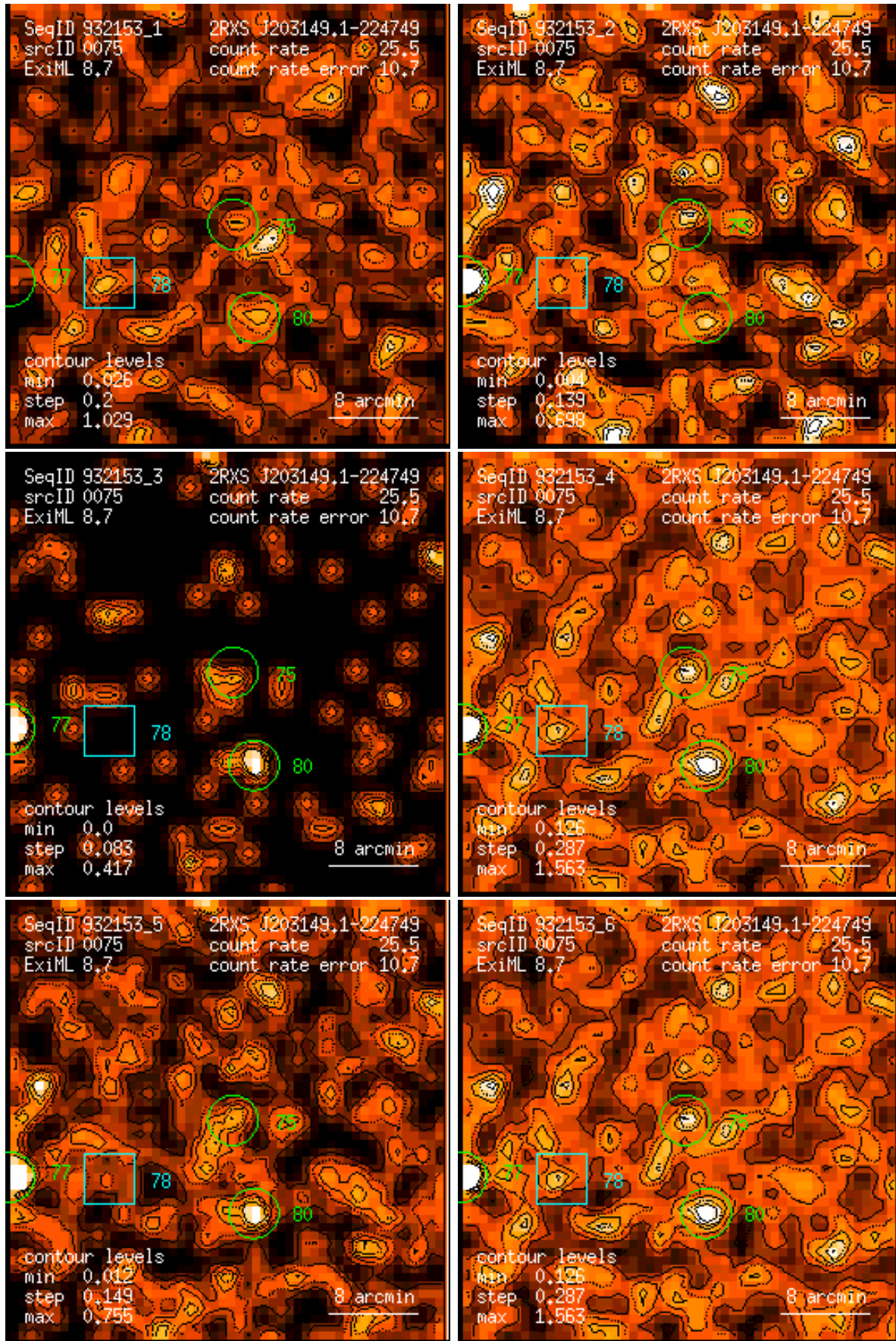
Figure 75: RASS 932153: detection 0075: band rate images, Gaussian filter: (1) PSPC channels 11 – 41, (2) 52 – 90, (3) 91 – 201, (4) 11 – 235, (5) 52 – 201, (6) 11 – 201. Broad band rates in counts/ks. Band rate contour levels in counts/ks/arcmin 2 .
