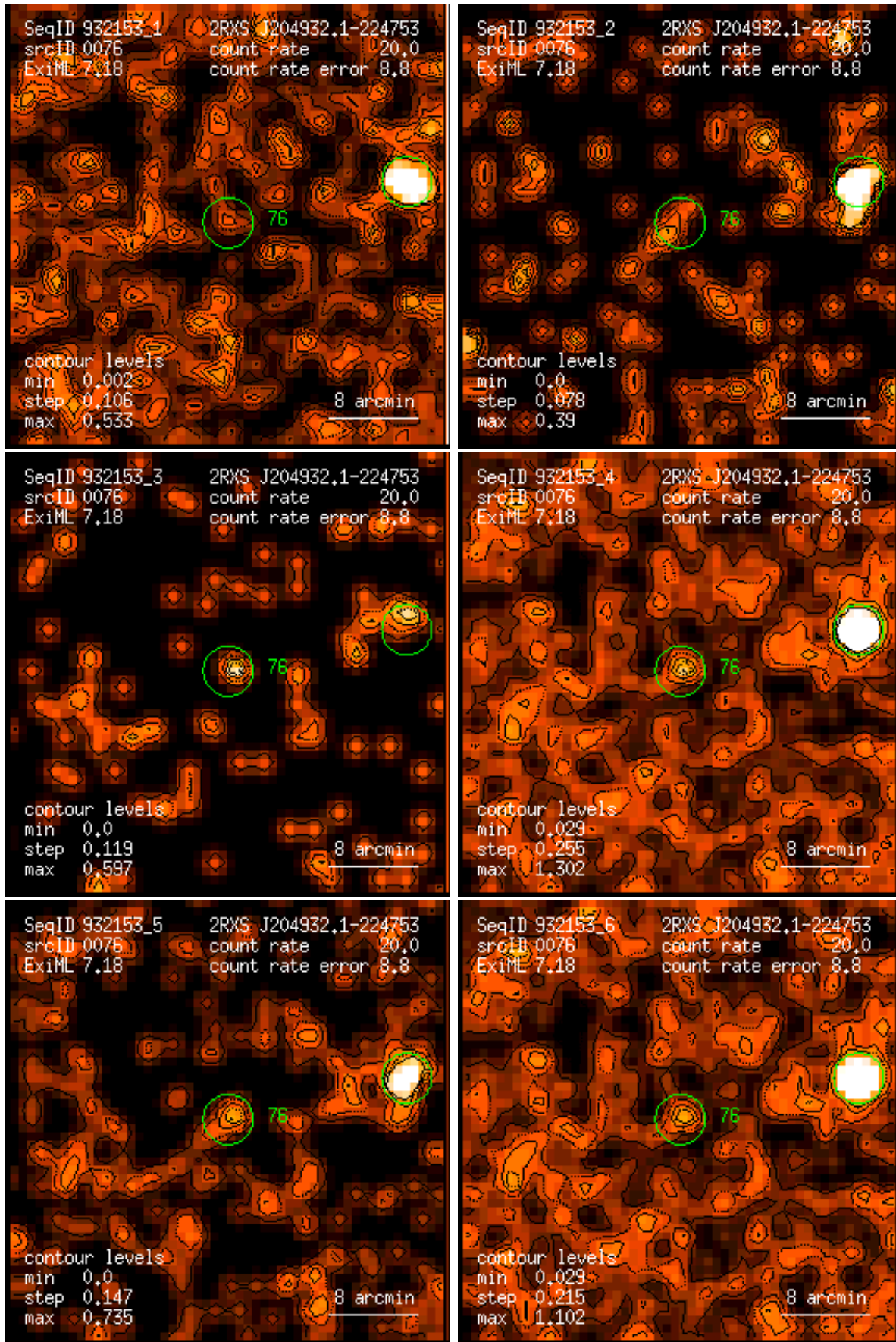
Figure 76: RASS 932153: detection 0076: band rate images, Gaussian filter: (1) PSPC channels 11 – 41, (2) 52 – 90, (3) 91 – 201, (4) 11 – 235, (5) 52 – 201, (6) 11 – 201. Broad band rates in counts/ks. Band rate contour levels in counts/ks/arcmin 2 .
