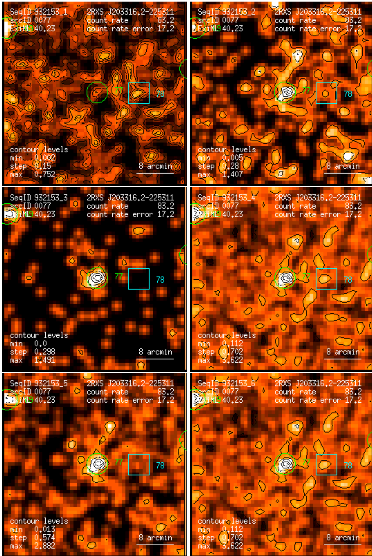
Figure 77: RASS 932153: detection 0077: band rate images, Gaussian filter: (1) PSPC channels 11 – 41, (2) 52 – 90, (3) 91 – 201, (4) 11 – 235, (5) 52 – 201, (6) 11 – 201. Broad band rates in counts/ks. Band rate contour levels in counts/ks/arcmin 2 .
