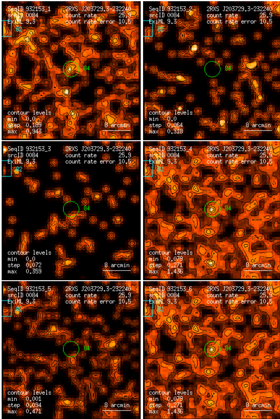
Figure 84: RASS 932153: detection 0084: band rate images, Gaussian filter: (1) PSPC channels 11 – 41, (2) 52 – 90, (3) 91 – 201, (4) 11 – 235, (5) 52 – 201, (6) 11 – 201. Broad band rates in counts/ks. Band rate contour levels in counts/ks/arcmin 2 .
