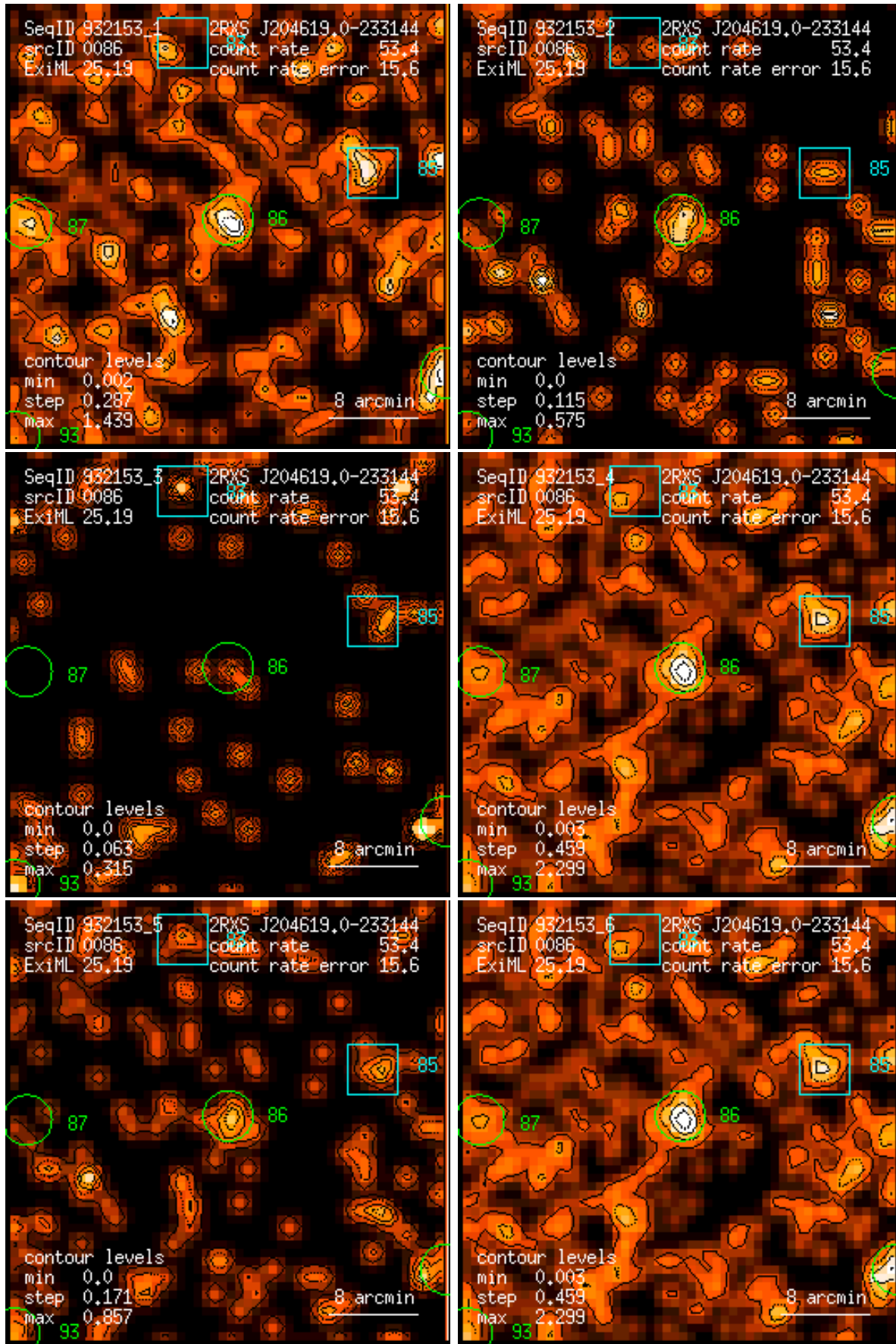
Figure 86: RASS 932153: detection 0086: band rate images, Gaussian filter: (1) PSPC channels 11 – 41, (2) 52 – 90, (3) 91 – 201, (4) 11 – 235, (5) 52 – 201, (6) 11 – 201. Broad band rates in counts/ks. Band rate contour levels in counts/ks/arcmin 2 .
