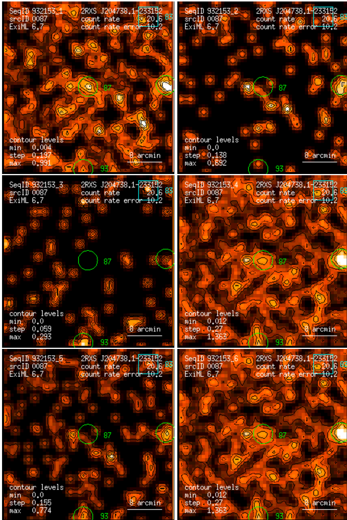
Figure 87: RASS 932153: detection 0087: band rate images, Gaussian filter: (1) PSPC channels 11 – 41, (2) 52 – 90, (3) 91 – 201, (4) 11 – 235, (5) 52 – 201, (6) 11 – 201. Broad band rates in counts/ks. Band rate contour levels in counts/ks/arcmin 2 .
