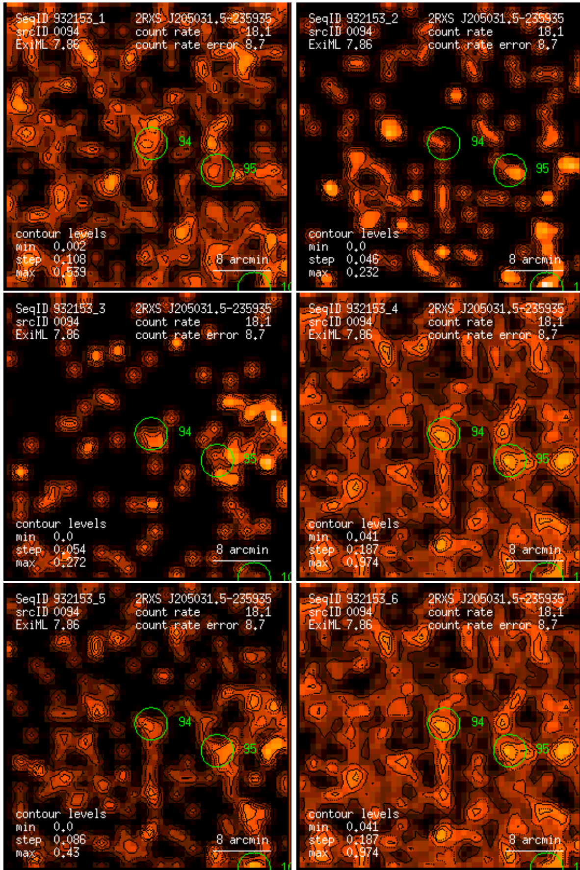
Figure 94: RASS 932153: detection 0094: band rate images, Gaussian filter: (1) PSPC channels 11 – 41, (2) 52 – 90, (3) 91 – 201, (4) 11 – 235, (5) 52 – 201, (6) 11 – 201. Broad band rates in counts/ks. Band rate contour levels in counts/ks/arcmin 2 .
