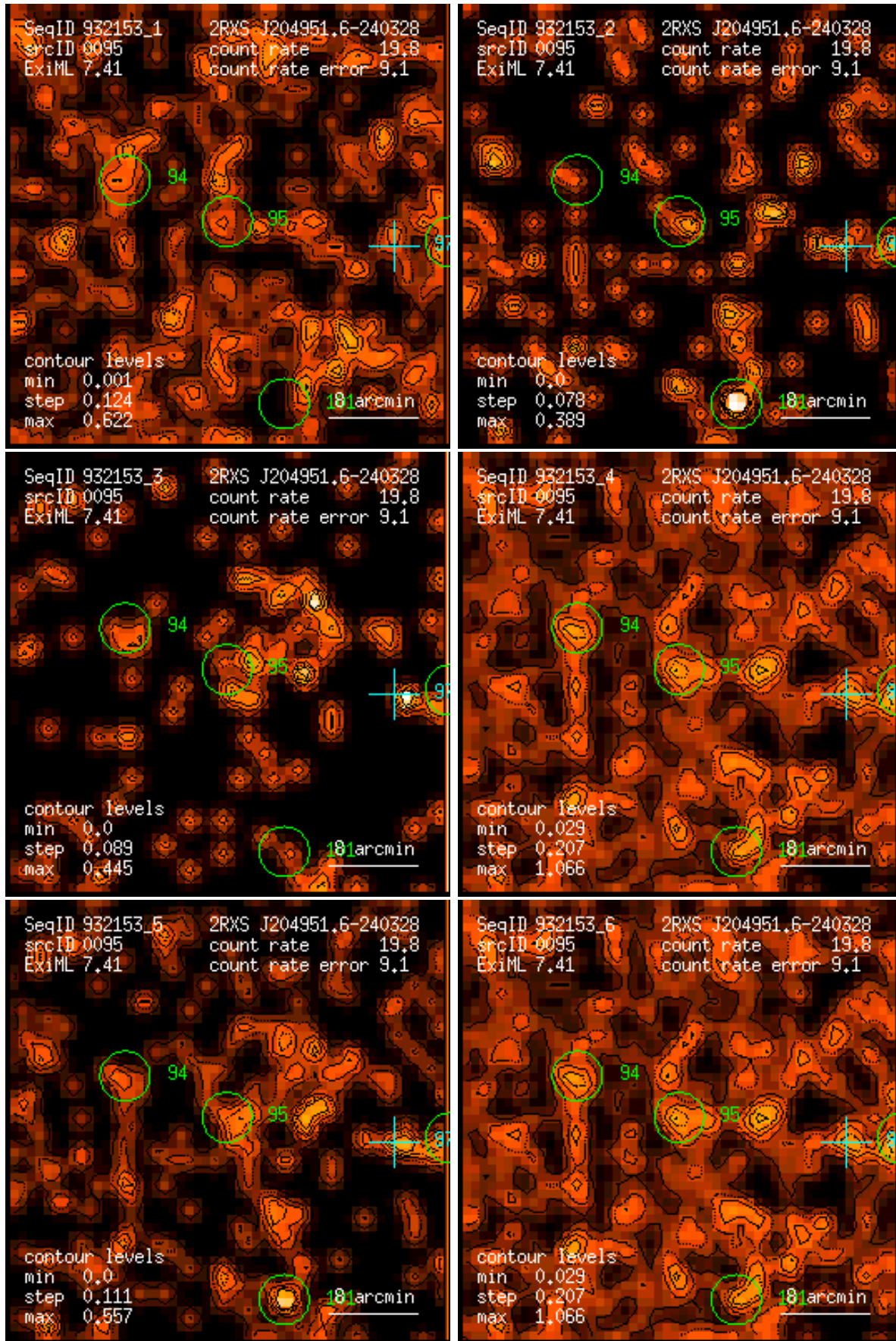
Figure 95: RASS 932153: detection 0095: band rate images, Gaussian filter: (1) PSPC channels 11 – 41, (2) 52 – 90, (3) 91 – 201, (4) 11 – 235, (5) 52 – 201, (6) 11 – 201. Broad band rates in counts/ks. Band rate contour levels in counts/ks/arcmin 2 .
