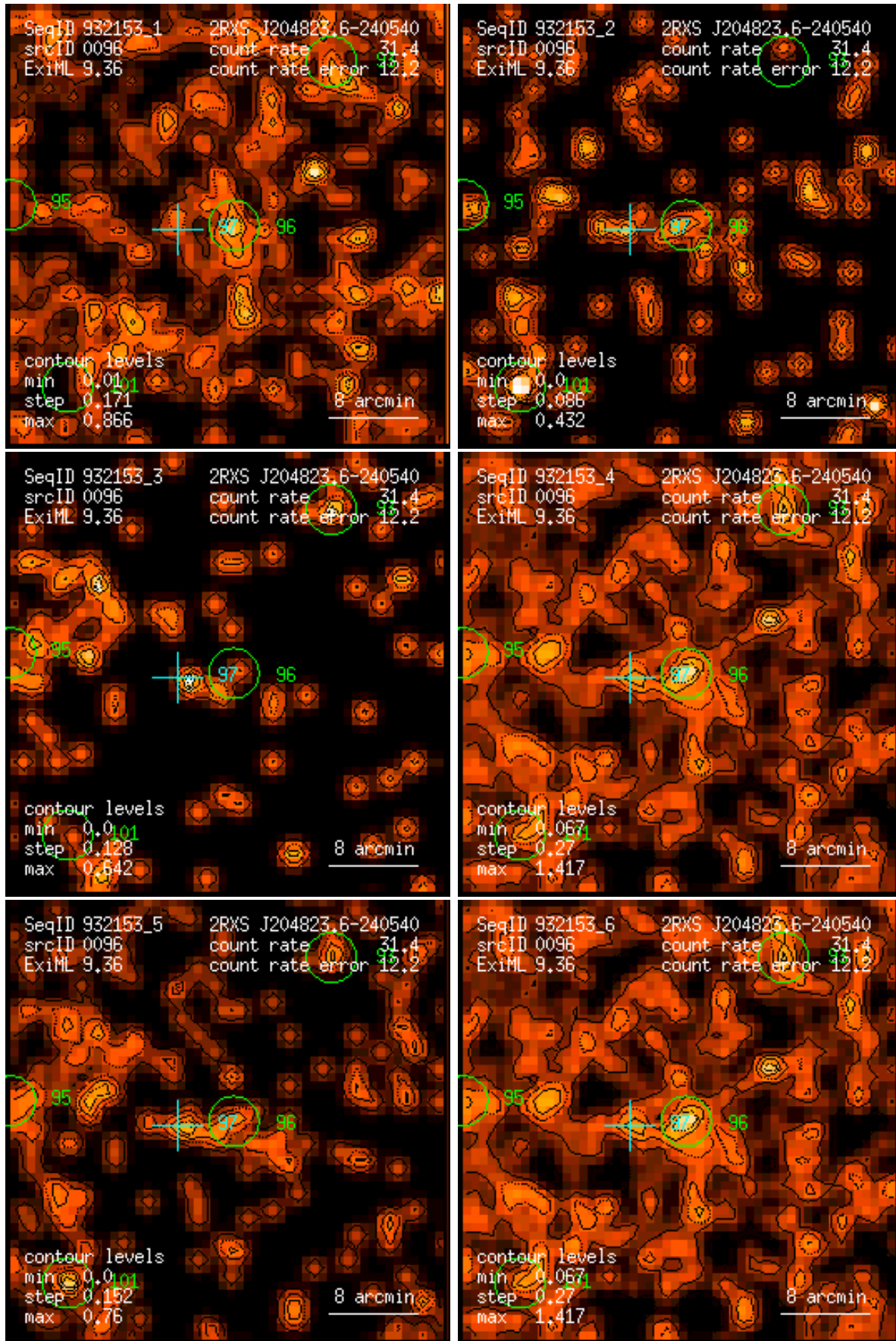
Figure 96: RASS 932153: detection 0096: band rate images, Gaussian filter: (1) PSPC channels 11 – 41, (2) 52 – 90, (3) 91 – 201, (4) 11 – 235, (5) 52 – 201, (6) 11 – 201. Broad band rates in counts/ks. Band rate contour levels in counts/ks/arcmin 2 .
