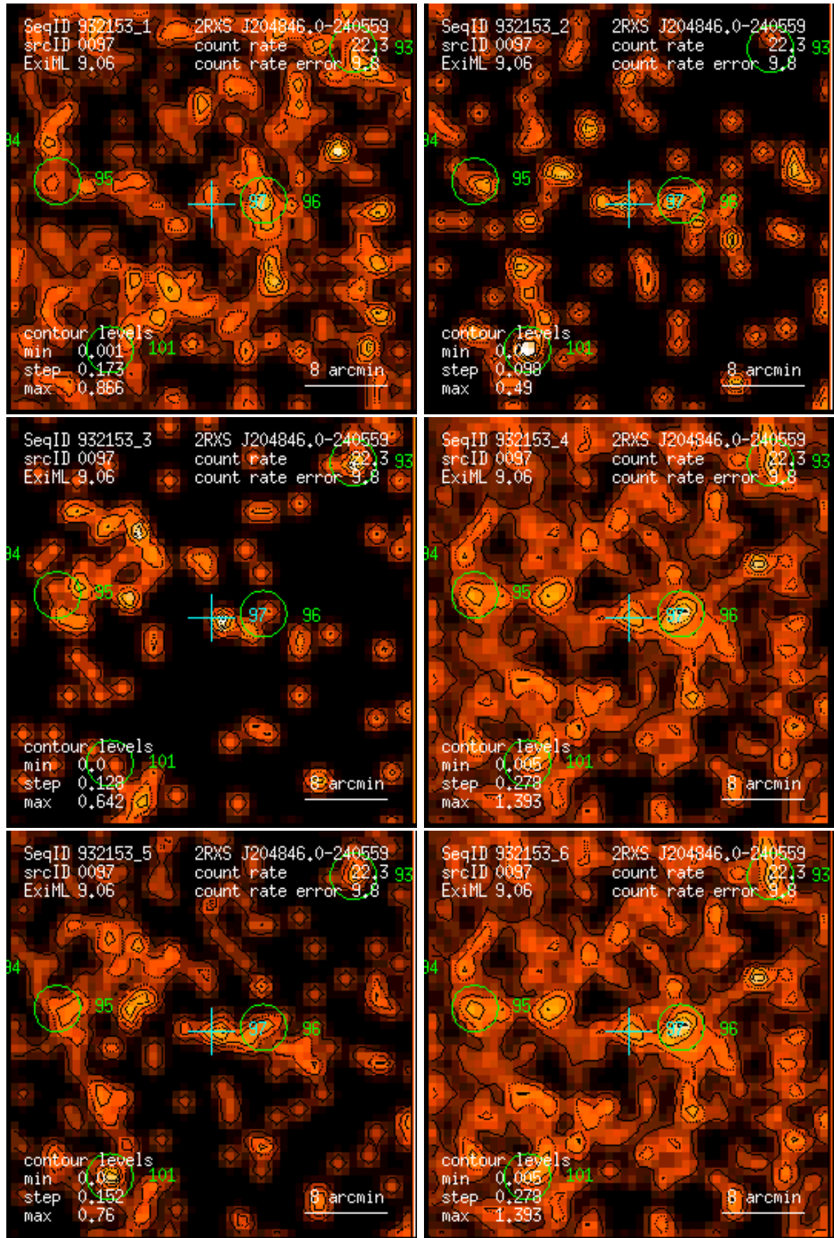
Figure 97: RASS 932153: detection 0097: band rate images, Gaussian filter: (1) PSPC channels 11 – 41, (2) 52 – 90, (3) 91 – 201, (4) 11 – 235, (5) 52 – 201, (6) 11 – 201. Broad band rates in counts/ks. Band rate contour levels in counts/ks/arcmin 2 .
