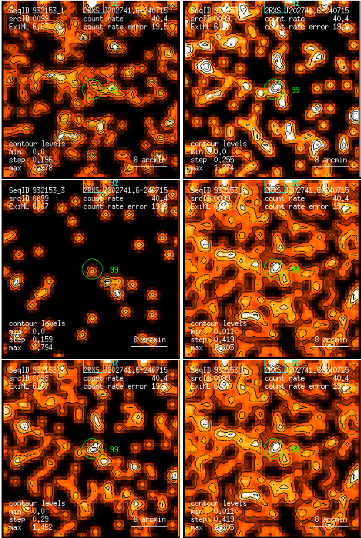
Figure 99: RASS 932153: detection 0099: band rate images, Gaussian filter: (1) PSPC channels 11 – 41, (2) 52 – 90, (3) 91 – 201, (4) 11 – 235, (5) 52 – 201, (6) 11 – 201. Broad band rates in counts/ks. Band rate contour levels in counts/ks/arcmin 2 .
