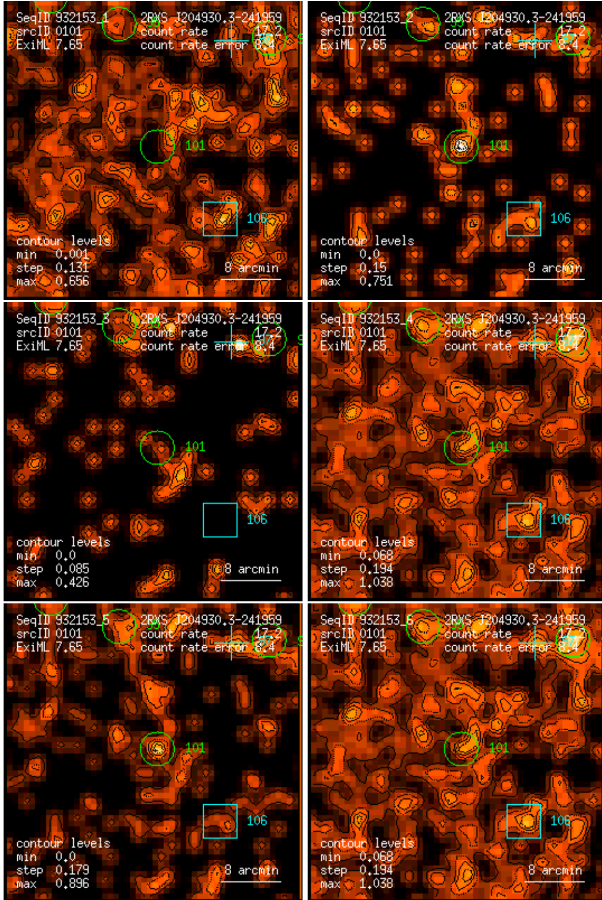
Figure 101: RASS 932153: detection 0101: band rate images, Gaussian filter: (1) PSPC channels 11 – 41, (2) 52 – 90, (3) 91 – 201, (4) 11 – 235, (5) 52 – 201, (6) 11 – 201. Broad band rates in counts/ks. Band rate contour levels in counts/ks/arcmin 2 .
