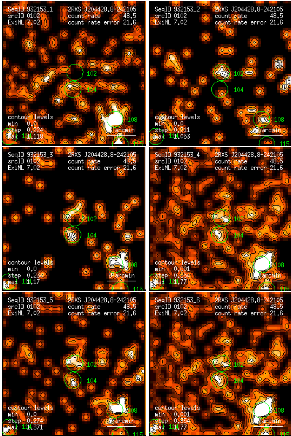
Figure 102: RASS 932153: detection 0102: band rate images, Gaussian filter: (1) PSPC channels 11 – 41, (2) 52 – 90, (3) 91 – 201, (4) 11 – 235, (5) 52 – 201, (6) 11 – 201. Broad band rates in counts/ks. Band rate contour levels in counts/ks/arcmin 2 .
