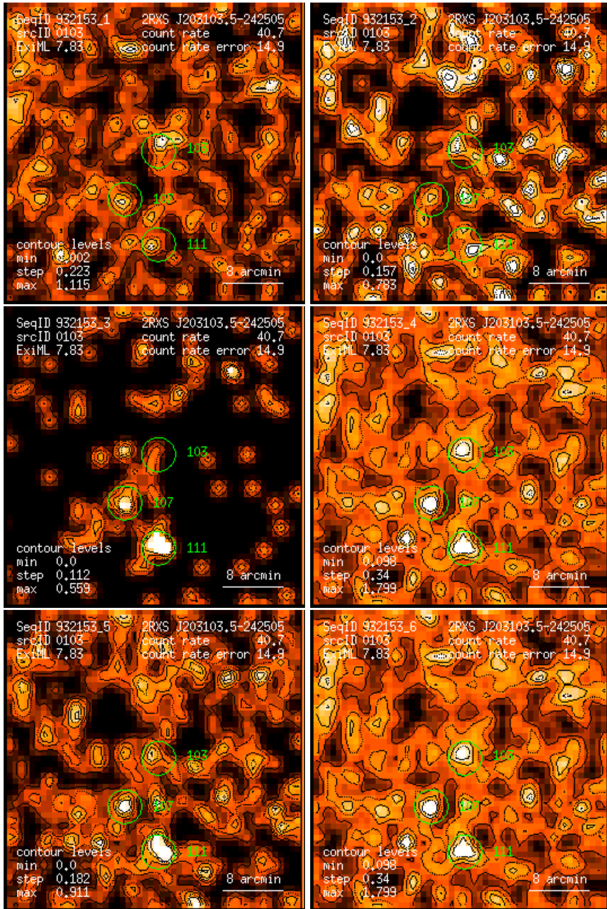
Figure 103: RASS 932153: detection 0103: band rate images, Gaussian filter: (1) PSPC channels 11 – 41, (2) 52 – 90, (3) 91 – 201, (4) 11 – 235, (5) 52 – 201, (6) 11 – 201. Broad band rates in counts/ks. Band rate contour levels in counts/ks/arcmin 2 .
