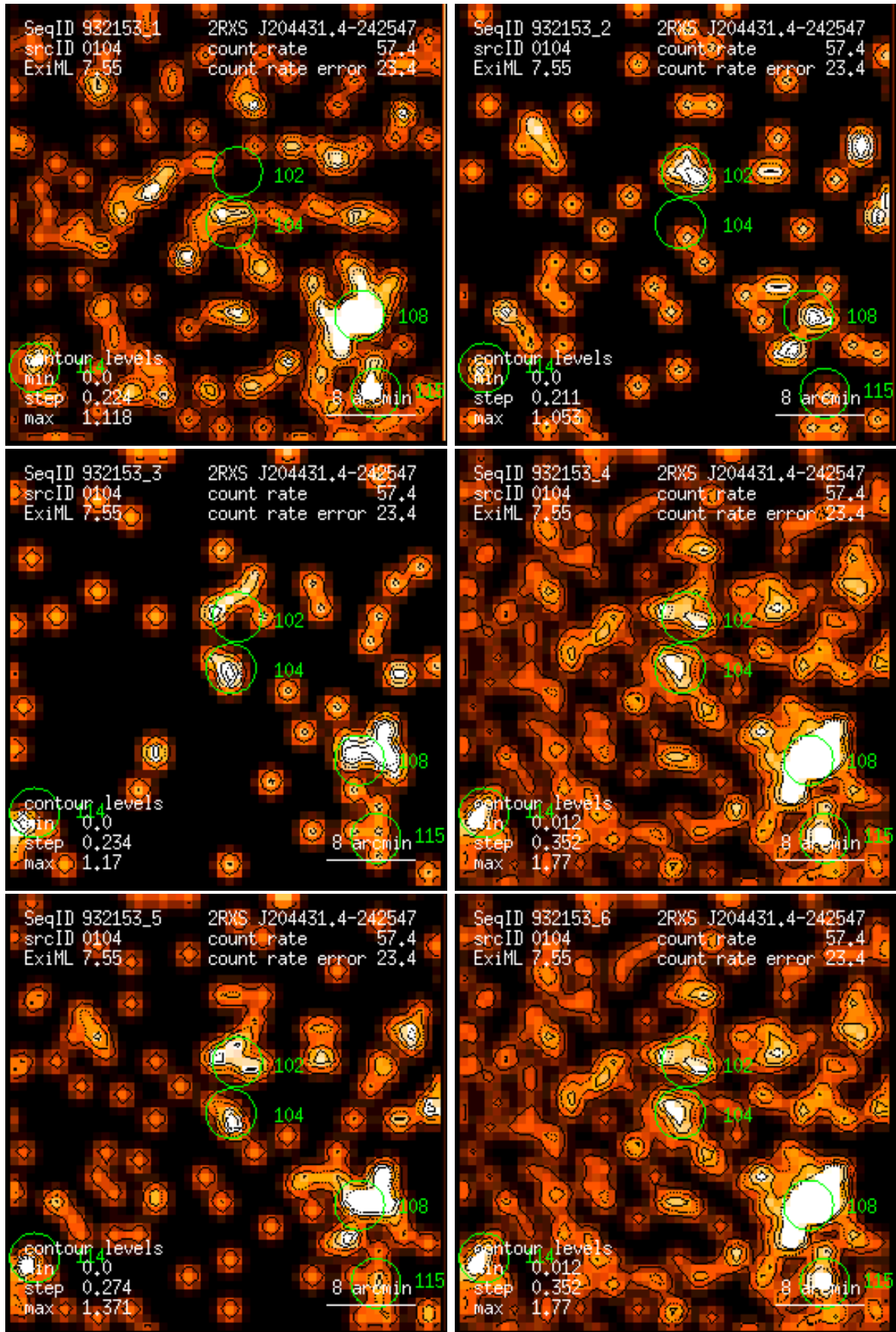
Figure 104: RASS 932153: detection 0104: band rate images, Gaussian filter: (1) PSPC channels 11 – 41, (2) 52 – 90, (3) 91 – 201, (4) 11 – 235, (5) 52 – 201, (6) 11 – 201. Broad band rates in counts/ks. Band rate contour levels in counts/ks/arcmin 2 .
