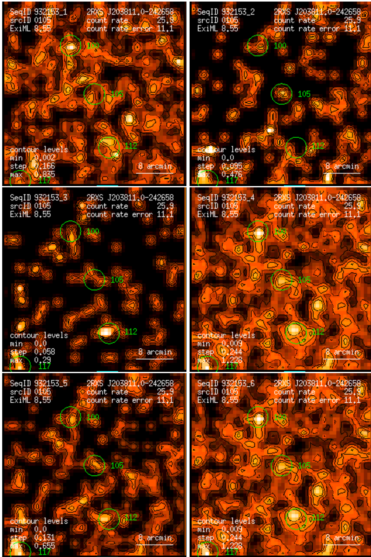
Figure 105: RASS 932153: detection 0105: band rate images, Gaussian filter: (1) PSPC channels 11 – 41, (2) 52 – 90, (3) 91 – 201, (4) 11 – 235, (5) 52 – 201, (6) 11 – 201. Broad band rates in counts/ks. Band rate contour levels in counts/ks/arcmin 2 .
