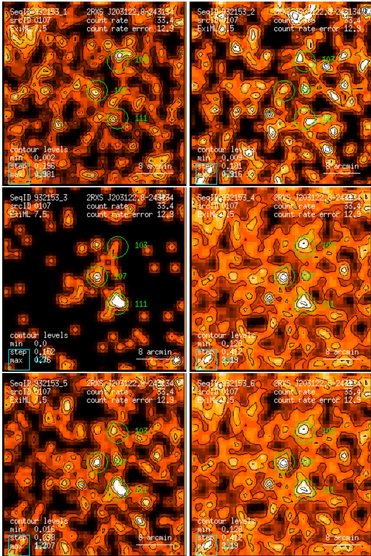
Figure 107: RASS 932153: detection 0107: band rate images, Gaussian filter: (1) PSPC channels 11 – 41, (2) 52 – 90, (3) 91 – 201, (4) 11 – 235, (5) 52 – 201, (6) 11 – 201. Broad band rates in counts/ks. Band rate contour levels in counts/ks/arcmin 2 .
