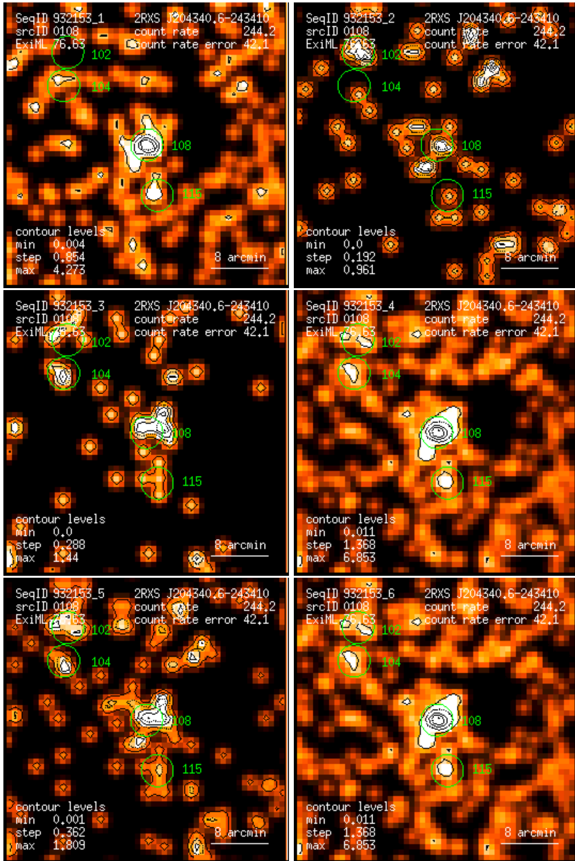
Figure 108: RASS 932153: detection 0108: band rate images, Gaussian filter: (1) PSPC channels 11 – 41, (2) 52 – 90, (3) 91 – 201, (4) 11 – 235, (5) 52 – 201, (6) 11 – 201. Broad band rates in counts/ks. Band rate contour levels in counts/ks/arcmin 2 .
