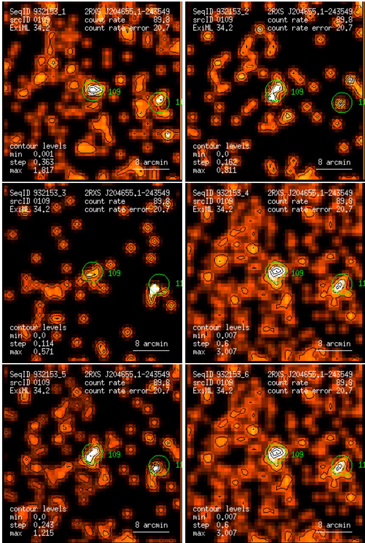
Figure 109: RASS 932153: detection 0109: band rate images, Gaussian filter: (1) PSPC channels 11 – 41, (2) 52 – 90, (3) 91 – 201, (4) 11 – 235, (5) 52 – 201, (6) 11 – 201. Broad band rates in counts/ks. Band rate contour levels in counts/ks/arcmin 2 .
