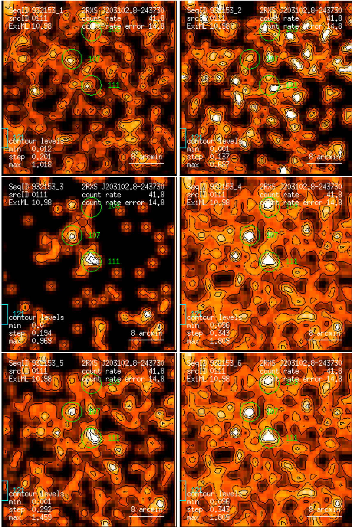
Figure 111: RASS 932153: detection 0111: band rate images, Gaussian filter: (1) PSPC channels 11 – 41, (2) 52 – 90, (3) 91 – 201, (4) 11 – 235, (5) 52 – 201, (6) 11 – 201. Broad band rates in counts/ks. Band rate contour levels in counts/ks/arcmin 2 .
