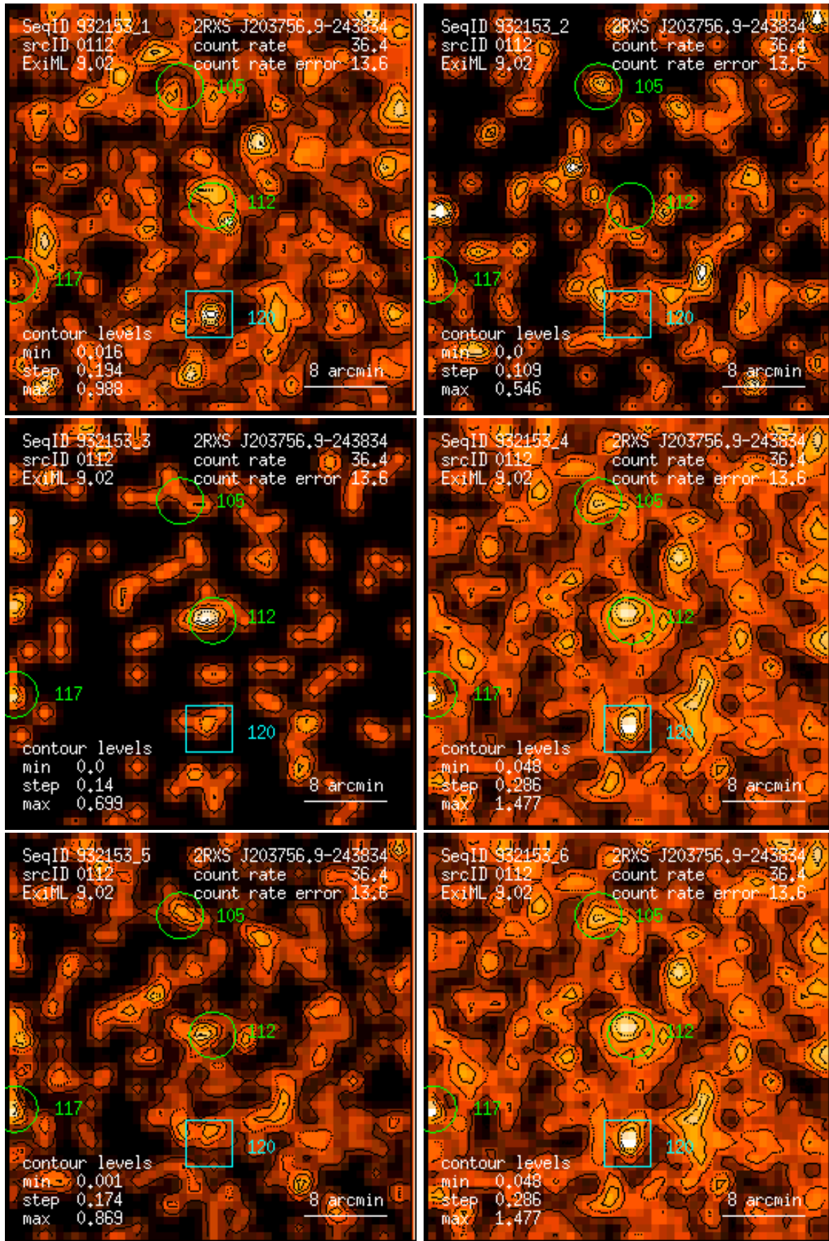
Figure 112: RASS 932153: detection 0112: band rate images, Gaussian filter: (1) PSPC channels 11 – 41, (2) 52 – 90, (3) 91 – 201, (4) 11 – 235, (5) 52 – 201, (6) 11 – 201. Broad band rates in counts/ks. Band rate contour levels in counts/ks/arcmin 2 .
