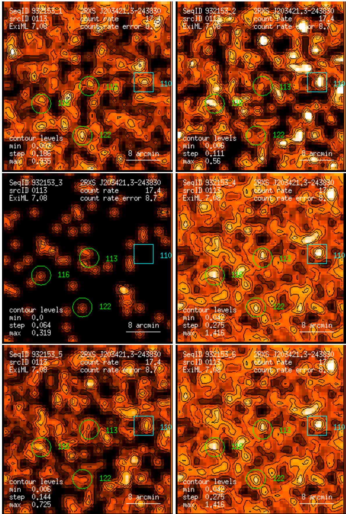
Figure 113: RASS 932153: detection 0113: band rate images, Gaussian filter: (1) PSPC channels 11 – 41, (2) 52 – 90, (3) 91 – 201, (4) 11 – 235, (5) 52 – 201, (6) 11 – 201. Broad band rates in counts/ks. Band rate contour levels in counts/ks/arcmin 2 .
