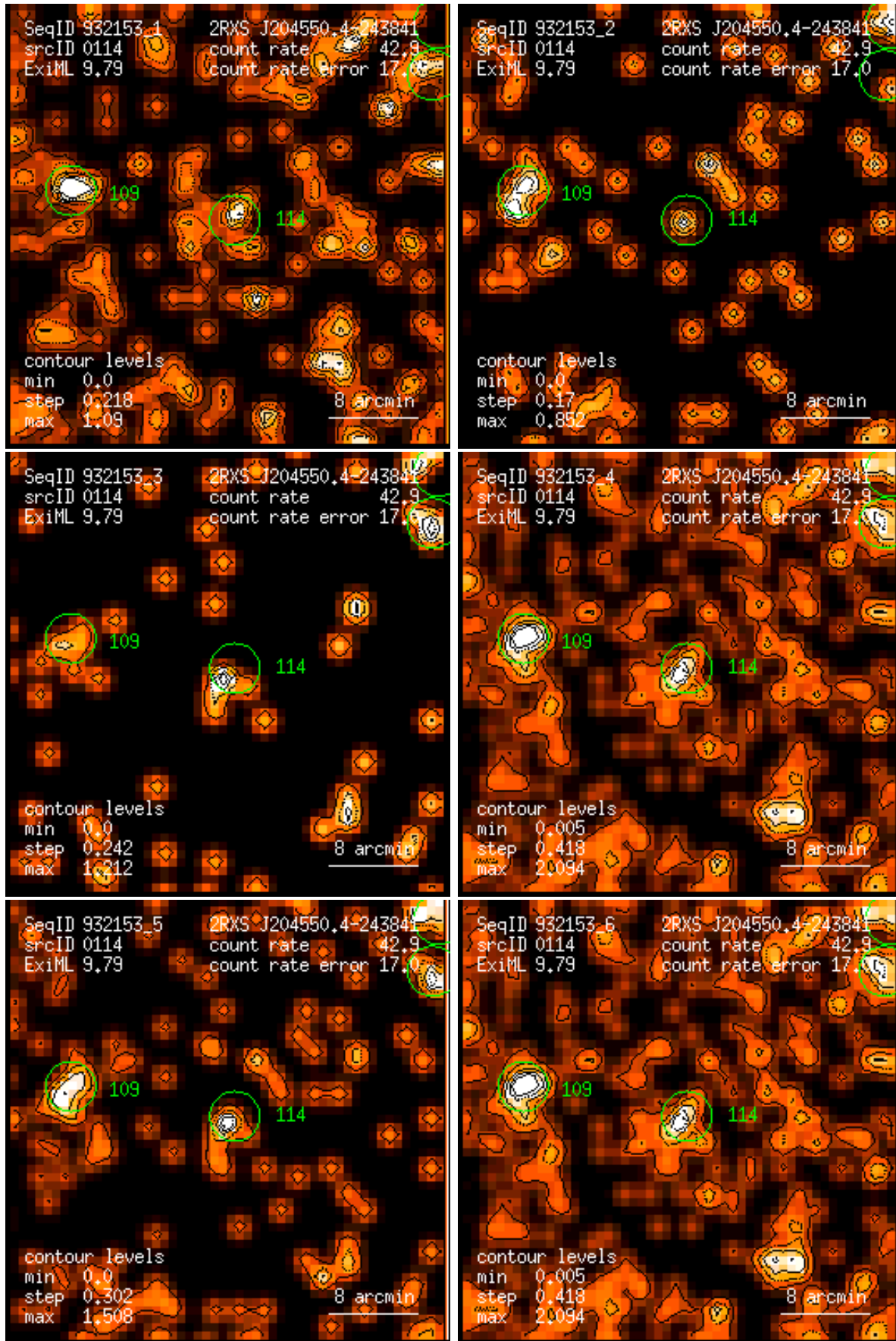
Figure 114: RASS 932153: detection 0114: band rate images, Gaussian filter: (1) PSPC channels 11 – 41, (2) 52 – 90, (3) 91 – 201, (4) 11 – 235, (5) 52 – 201, (6) 11 – 201. Broad band rates in counts/ks. Band rate contour levels in counts/ks/arcmin 2 .
