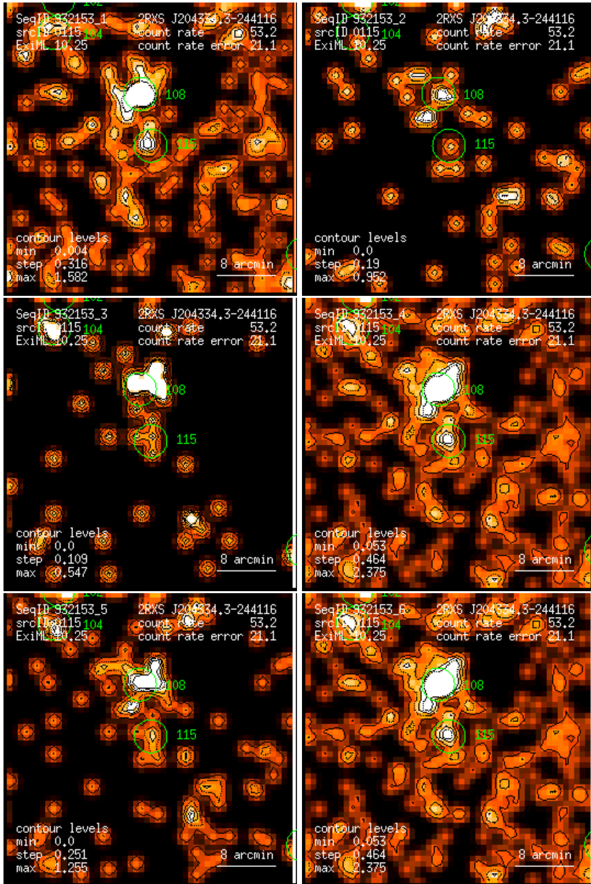
Figure 115: RASS 932153: detection 0115: band rate images, Gaussian filter: (1) PSPC channels 11 – 41, (2) 52 – 90, (3) 91 – 201, (4) 11 – 235, (5) 52 – 201, (6) 11 – 201. Broad band rates in counts/ks. Band rate contour levels in counts/ks/arcmin 2 .
