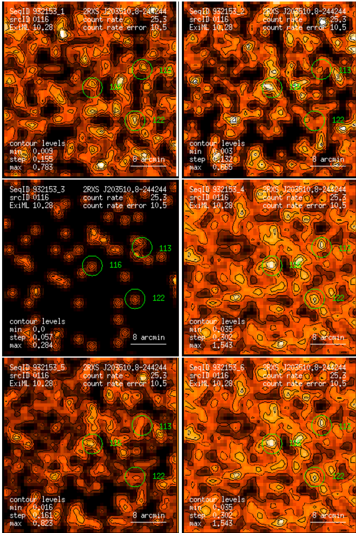
Figure 116: RASS 932153: detection 0116: band rate images, Gaussian filter: (1) PSPC channels 11 – 41, (2) 52 – 90, (3) 91 – 201, (4) 11 – 235, (5) 52 – 201, (6) 11 – 201. Broad band rates in counts/ks. Band rate contour levels in counts/ks/arcmin 2 .
