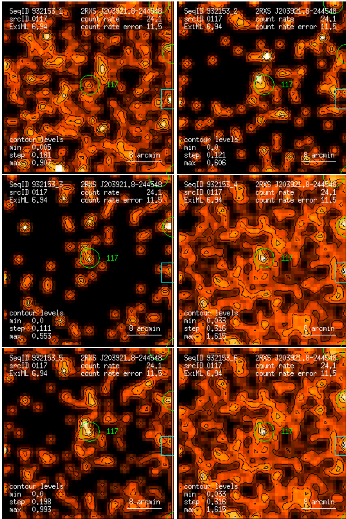
Figure 117: RASS 932153: detection 0117: band rate images, Gaussian filter: (1) PSPC channels 11 – 41, (2) 52 – 90, (3) 91 – 201, (4) 11 – 235, (5) 52 – 201, (6) 11 – 201. Broad band rates in counts/ks. Band rate contour levels in counts/ks/arcmin 2 .
