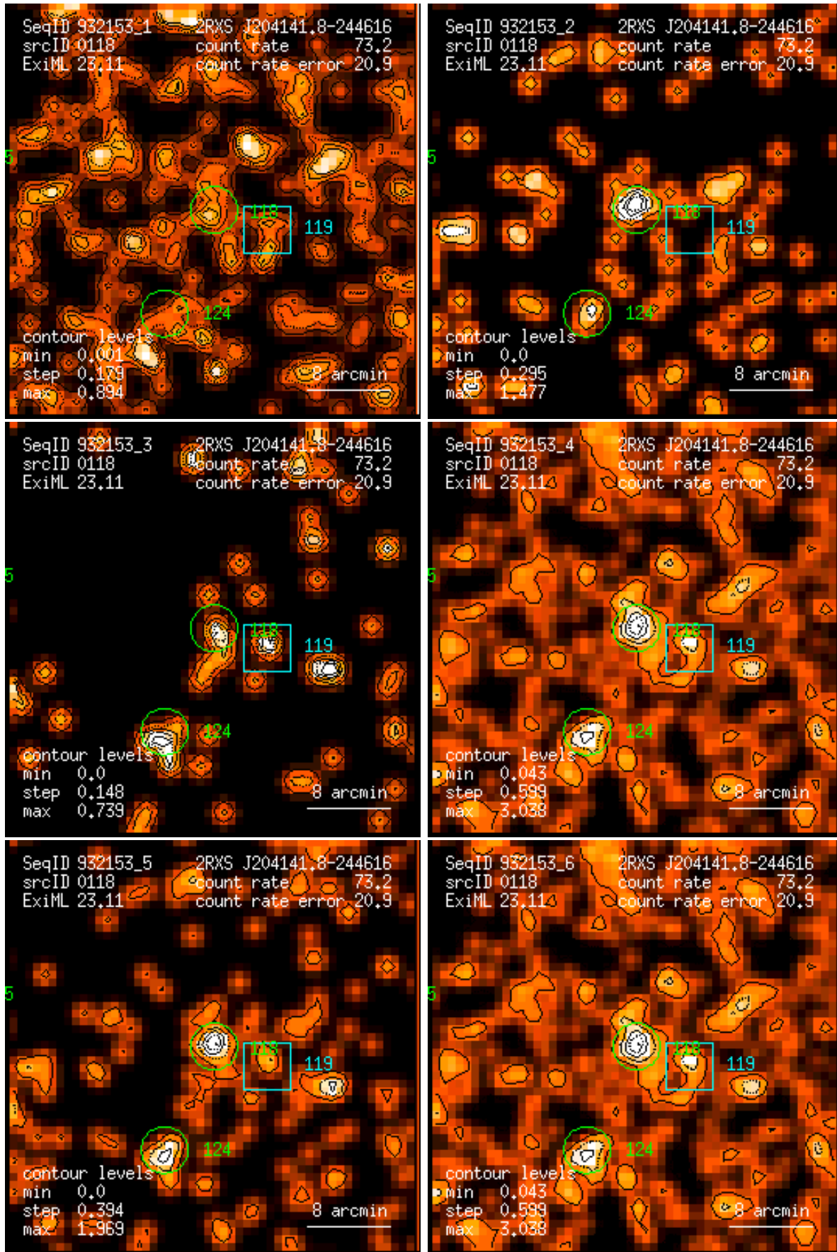
Figure 118: RASS 932153: detection 0118: band rate images, Gaussian filter: (1) PSPC channels 11 – 41, (2) 52 – 90, (3) 91 – 201, (4) 11 – 235, (5) 52 – 201, (6) 11 – 201. Broad band rates in counts/ks. Band rate contour levels in counts/ks/arcmin 2 .
