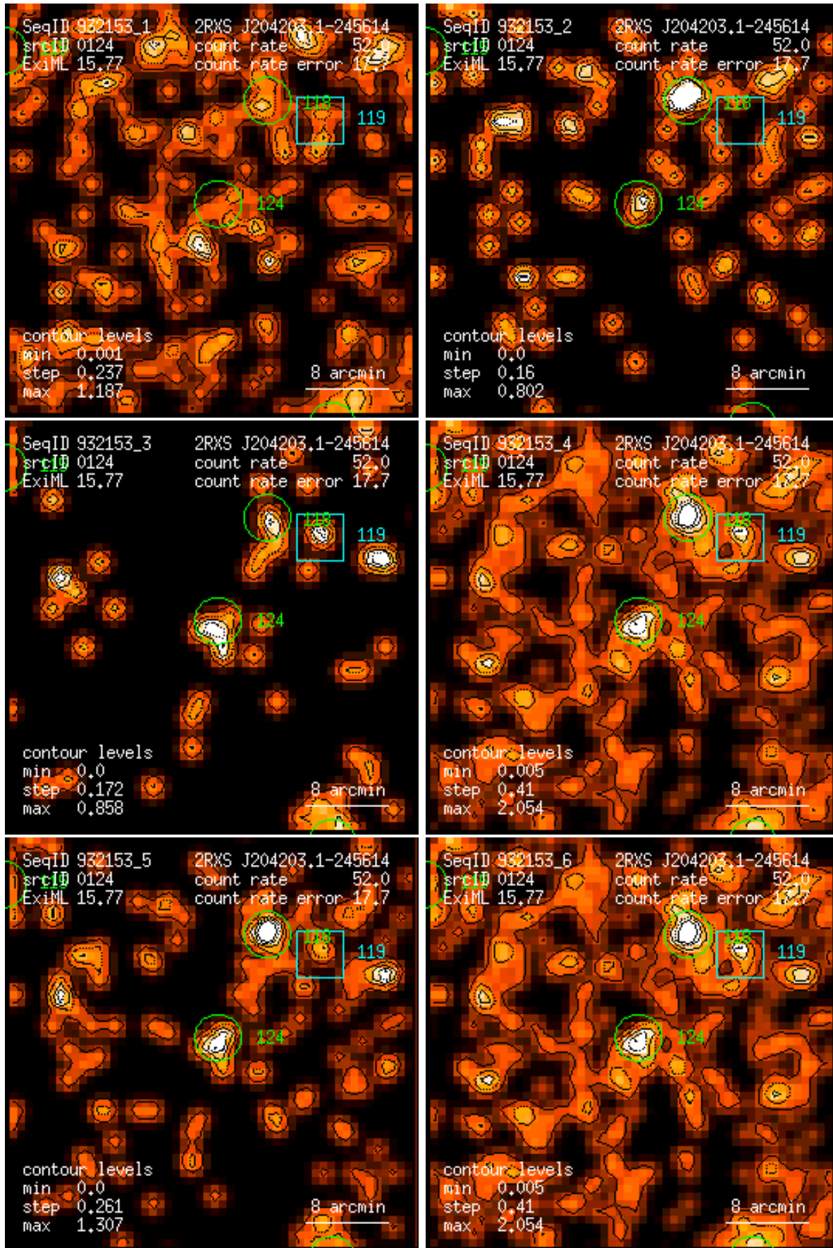
Figure 124: RASS 932153: detection 0124: band rate images, Gaussian filter: (1) PSPC channels 11 – 41, (2) 52 – 90, (3) 91 – 201, (4) 11 – 235, (5) 52 – 201, (6) 11 – 201. Broad band rates in counts/ks. Band rate contour levels in counts/ks/arcmin 2 .
