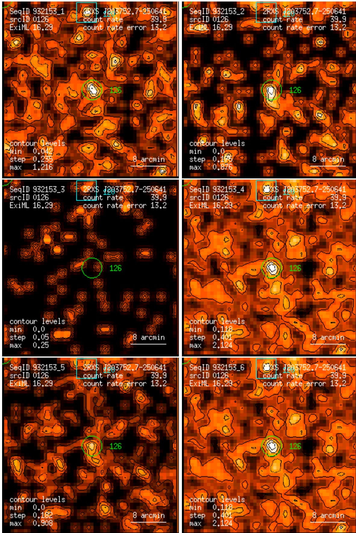
Figure 126: RASS 932153: detection 0126: band rate images, Gaussian filter: (1) PSPC channels 11 – 41, (2) 52 – 90, (3) 91 – 201, (4) 11 – 235, (5) 52 – 201, (6) 11 – 201. Broad band rates in counts/ks. Band rate contour levels in counts/ks/arcmin 2 .
