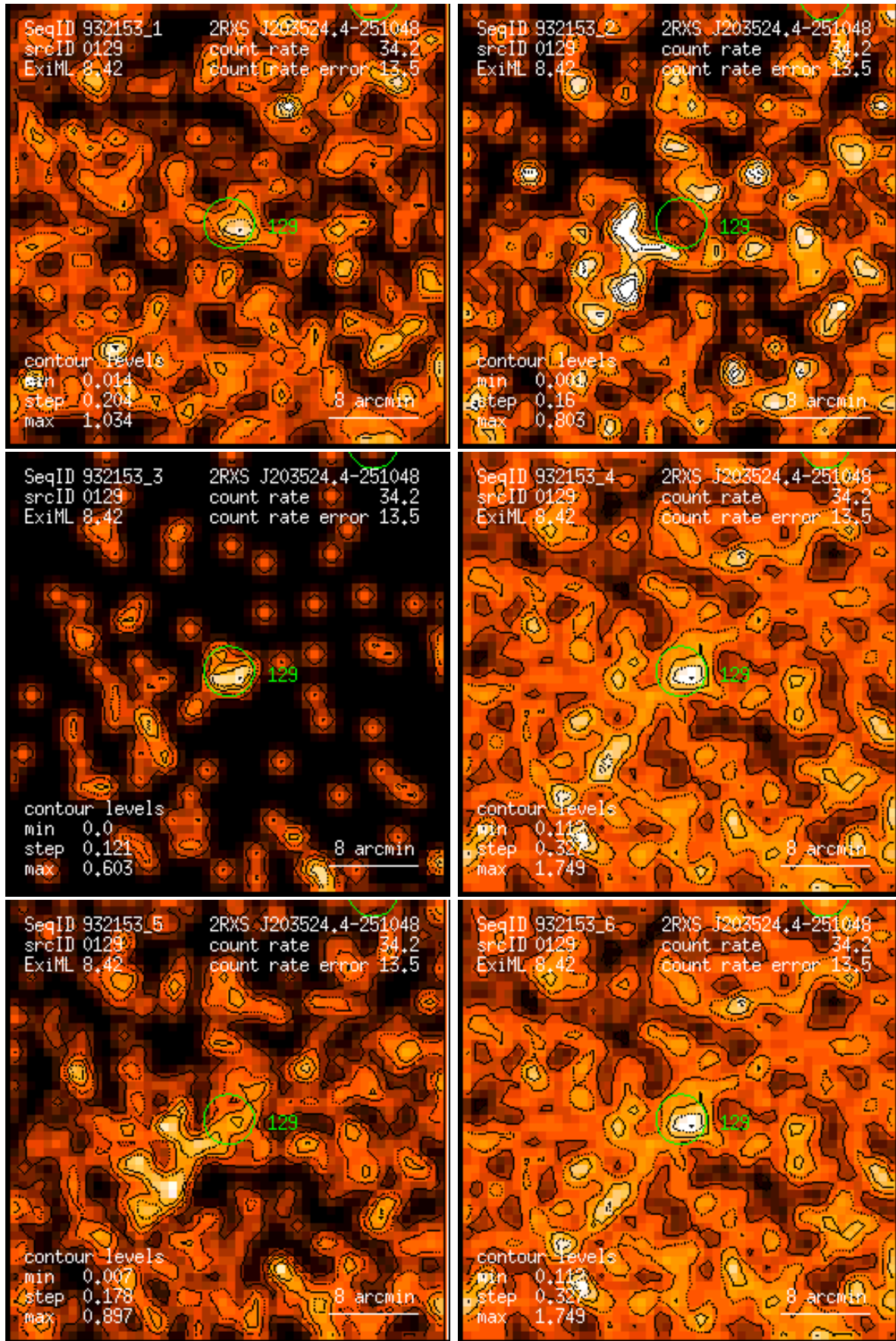
Figure 129: RASS 932153: detection 0129: band rate images, Gaussian filter: (1) PSPC channels 11 – 41, (2) 52 – 90, (3) 91 – 201, (4) 11 – 235, (5) 52 – 201, (6) 11 – 201. Broad band rates in counts/ks. Band rate contour levels in counts/ks/arcmin 2 .
