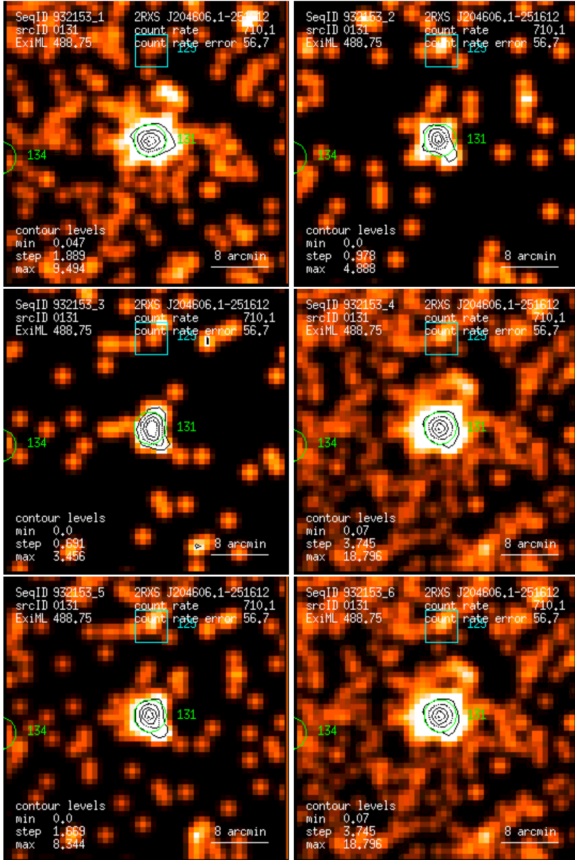
Figure 131: RASS 932153: detection 0131: band rate images, Gaussian filter: (1) PSPC channels 11 – 41, (2) 52 – 90, (3) 91 – 201, (4) 11 – 235, (5) 52 – 201, (6) 11 – 201. Broad band rates in counts/ks. Band rate contour levels in counts/ks/arcmin 2 .
